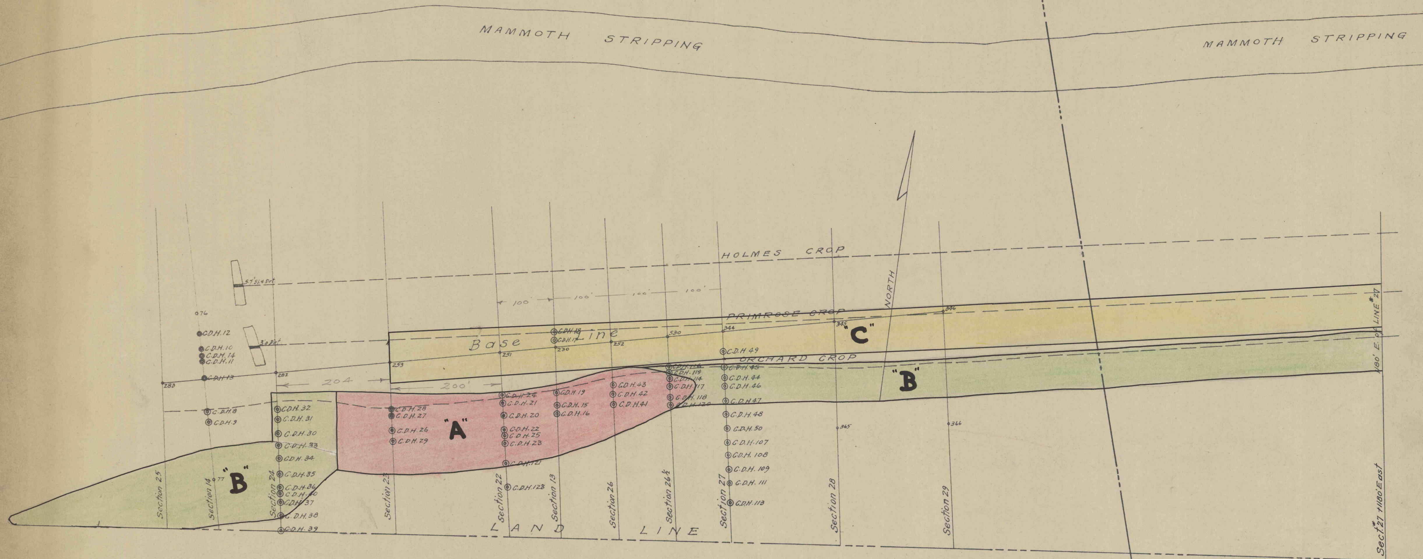
Plan Showing Provings for Proposed Stripping of Veins Overlying the Mammoth Merriam Section of Germantown Colliery Engineering Dept. Raven Run Coal Co. Jeddo, Pa. Scale 1"=100' Sept. 6, 1943.
