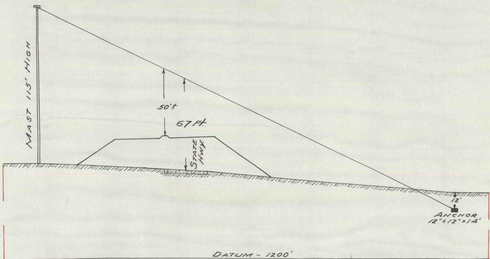
PROFILE ON GUY LINE TO ANCHOR N°2
