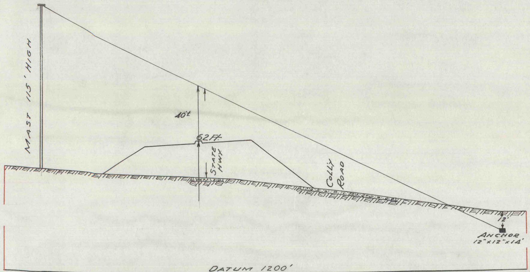
PROFILE ON GUY LINE TO ANCHOR N°1
