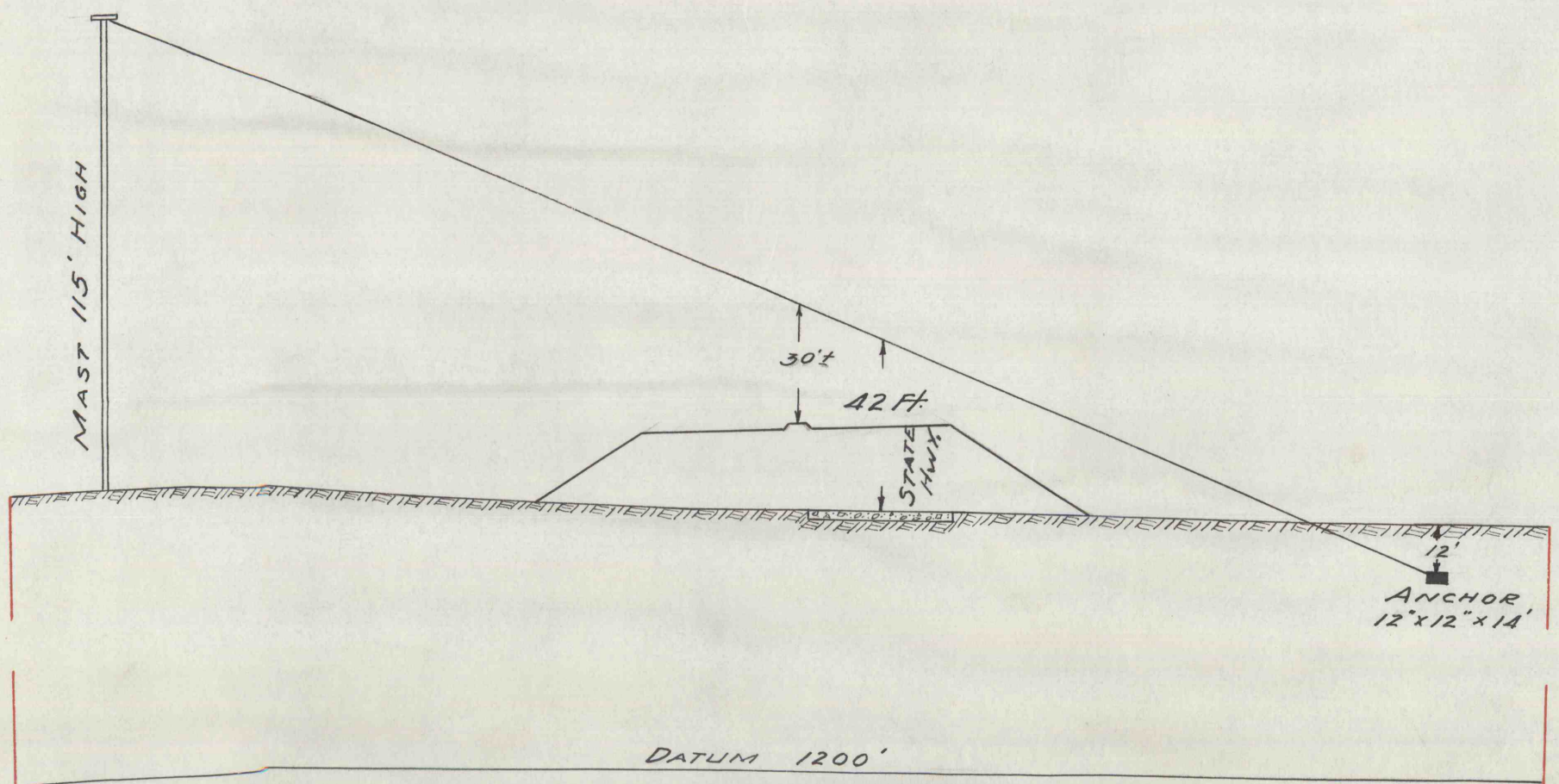
PROFILE ON GUY LINE TO ANCHOR N°3
