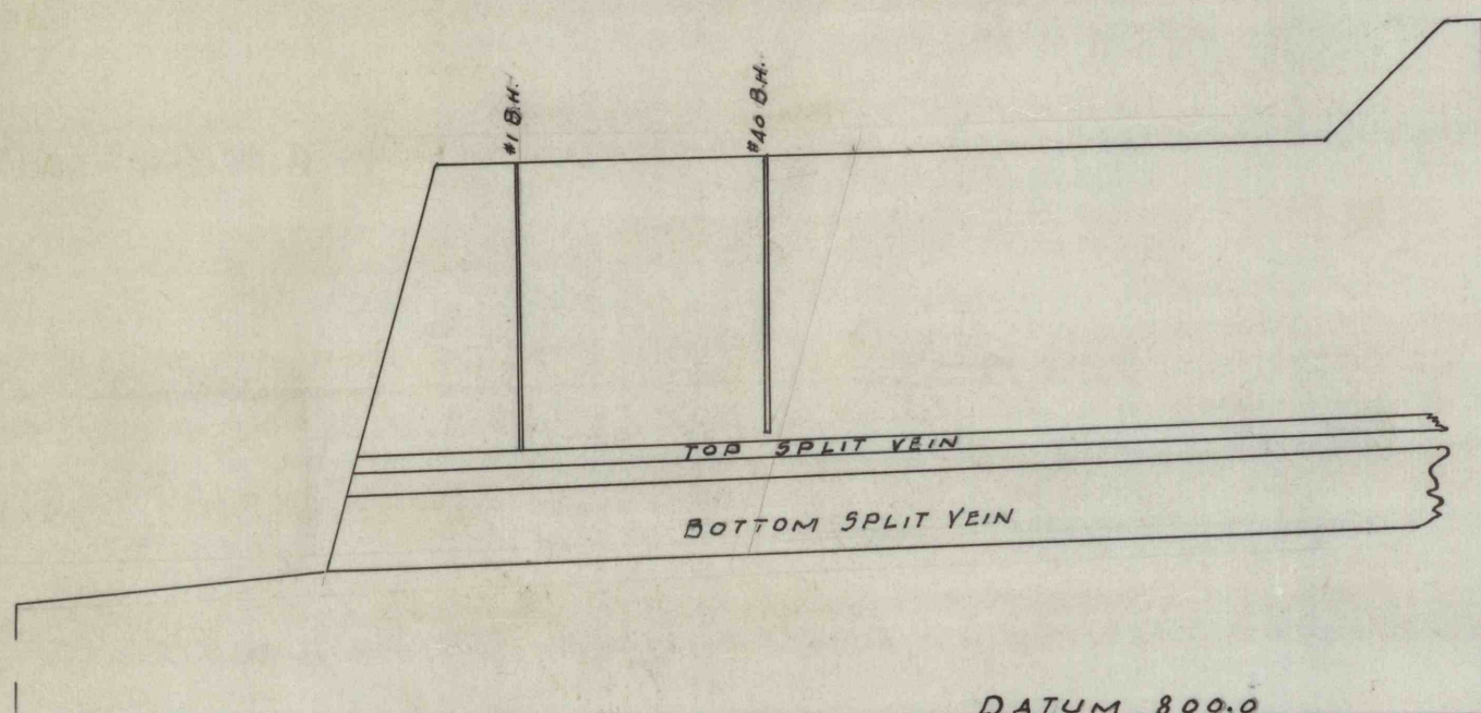
LONGITUDINAL SECTION THROUGH #1 BLAST HOLE LOOKING NORTH SCALE 1"=50'
