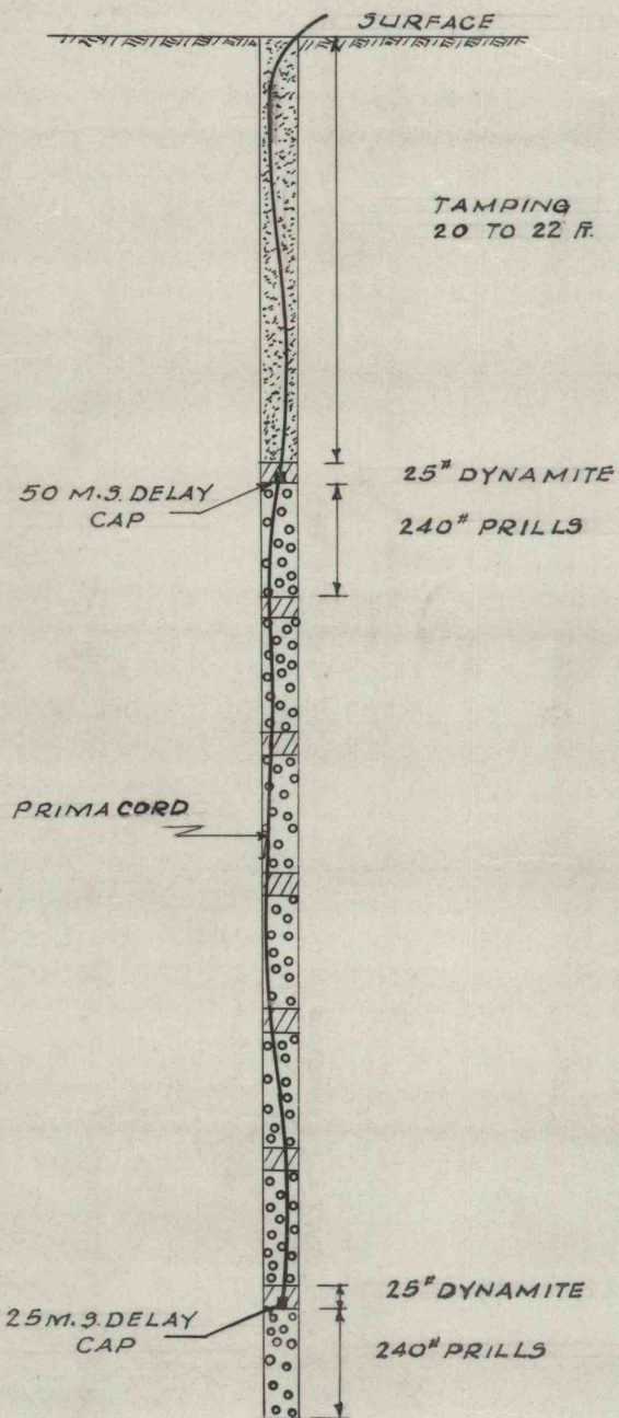
TYPICAL SECTION SHOWING METHOD OF LOADING 12" DIA. BLAST HOLES
