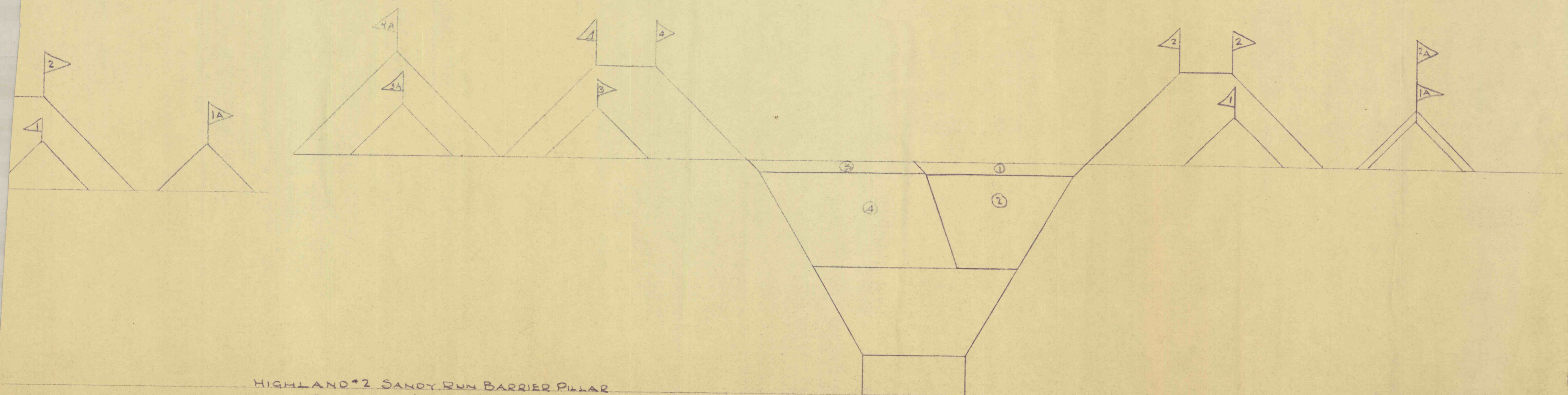
SECT*1 LONG*4 NORTH PIT 1"=50' LOOKING NORTH
