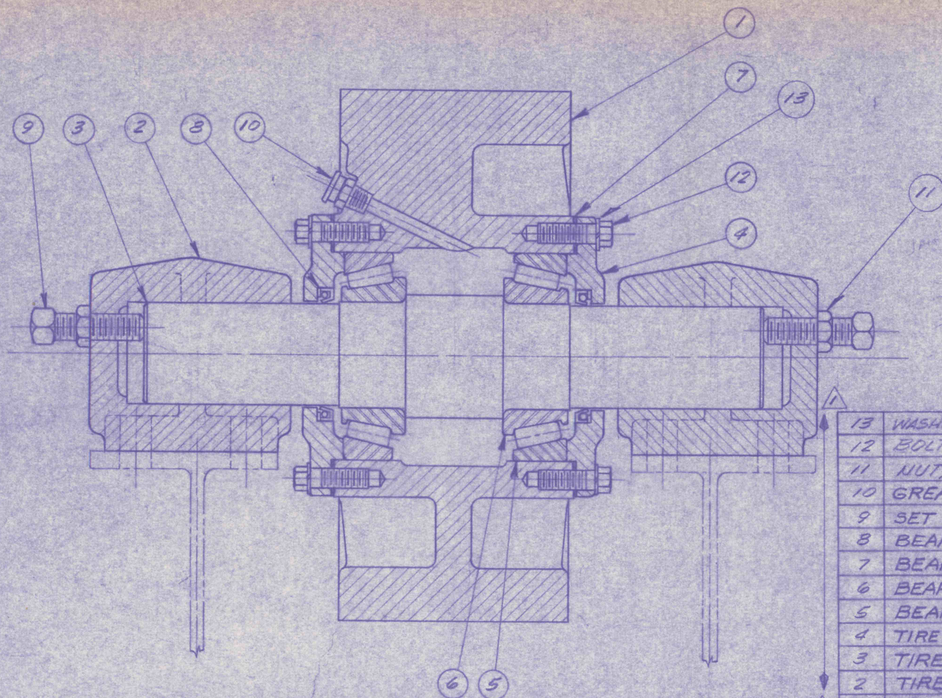
TIRE ROLLER ASSEMBLY ~ #42132A
