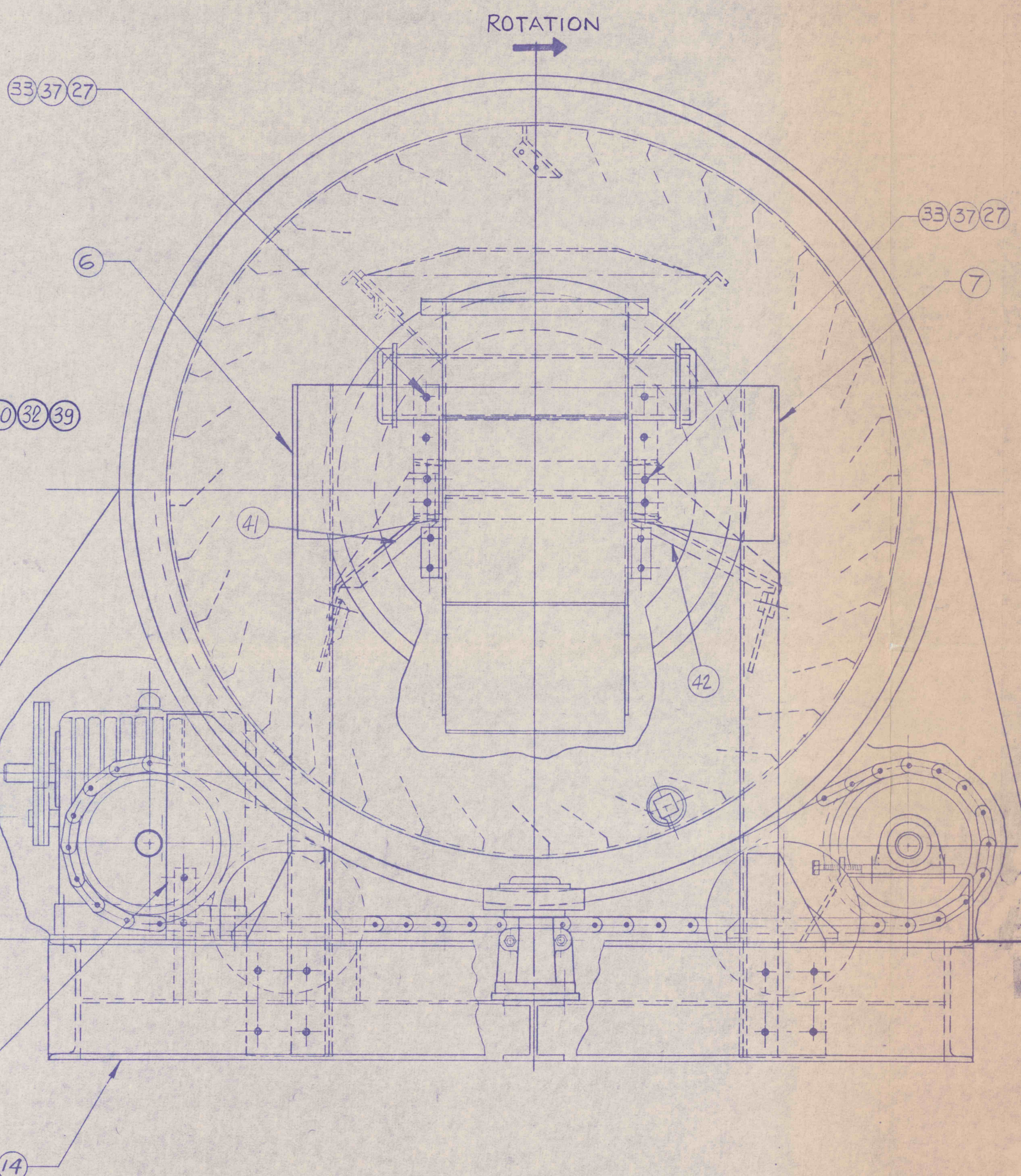
VIEW "B"
