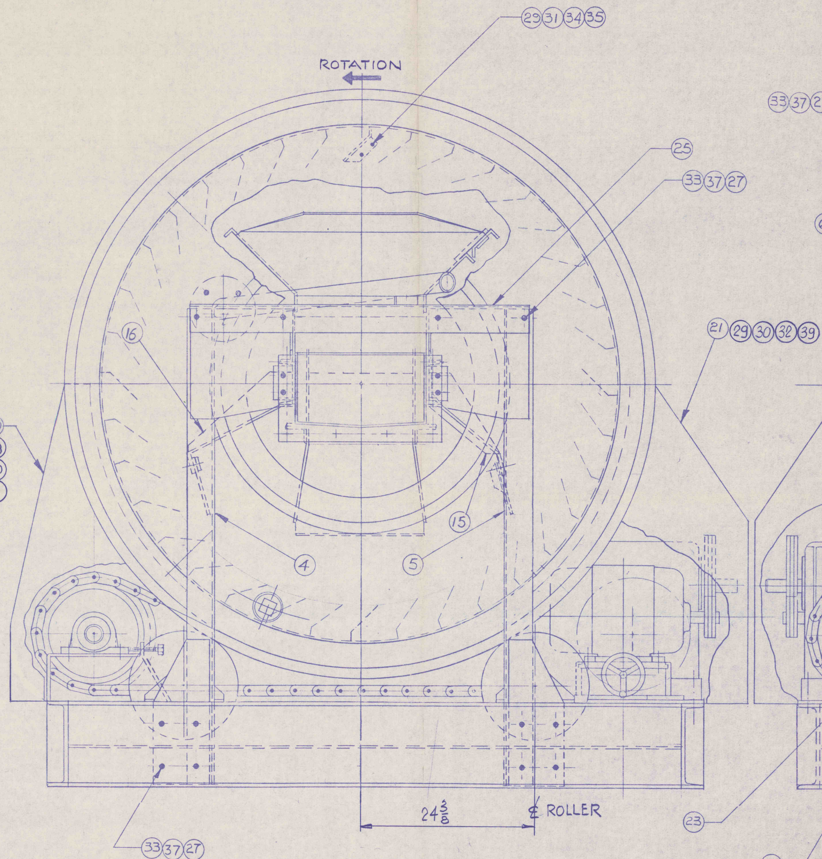
VIEW "D"
