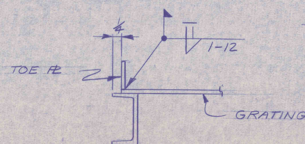
SECT. K-K
