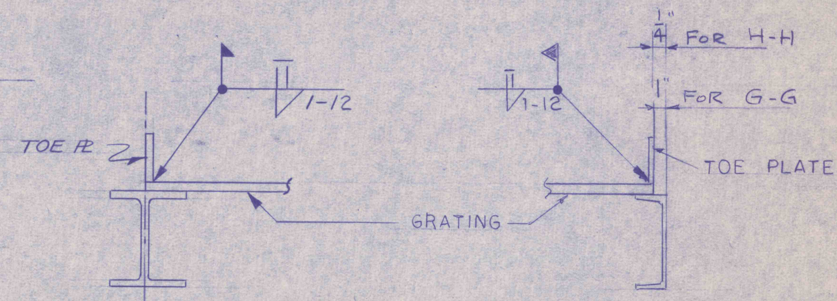
SECT. K-K
