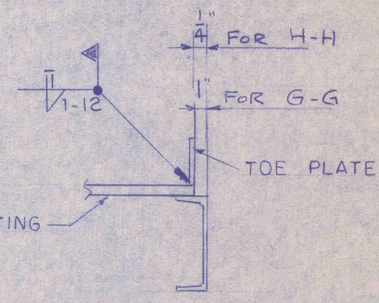
SECT. G-G
