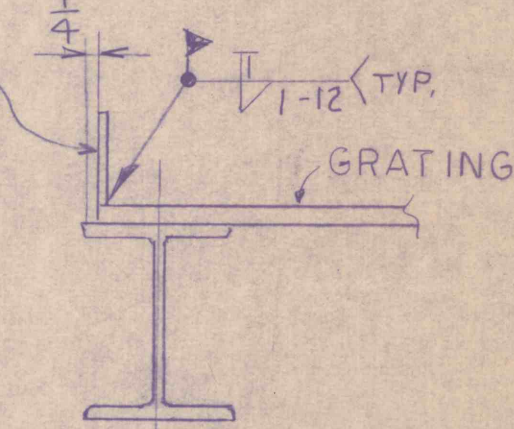
SECT. F-F
