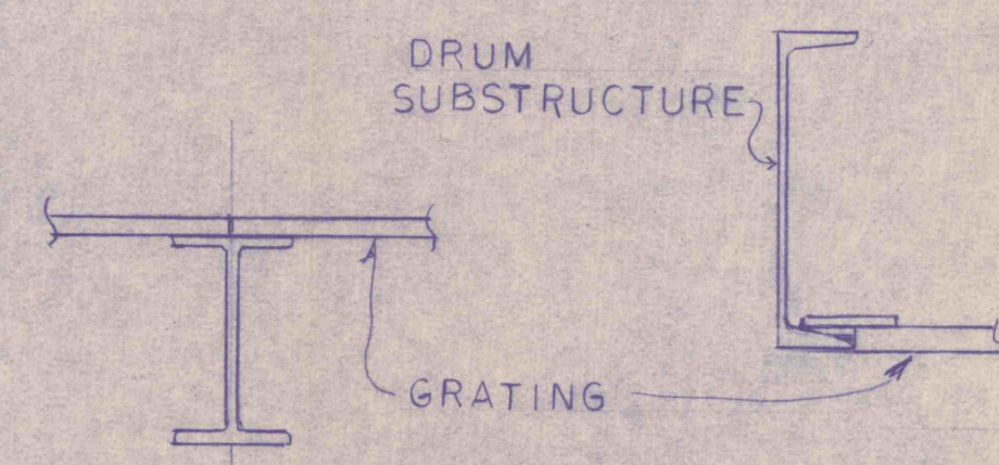
SECT. D-D
