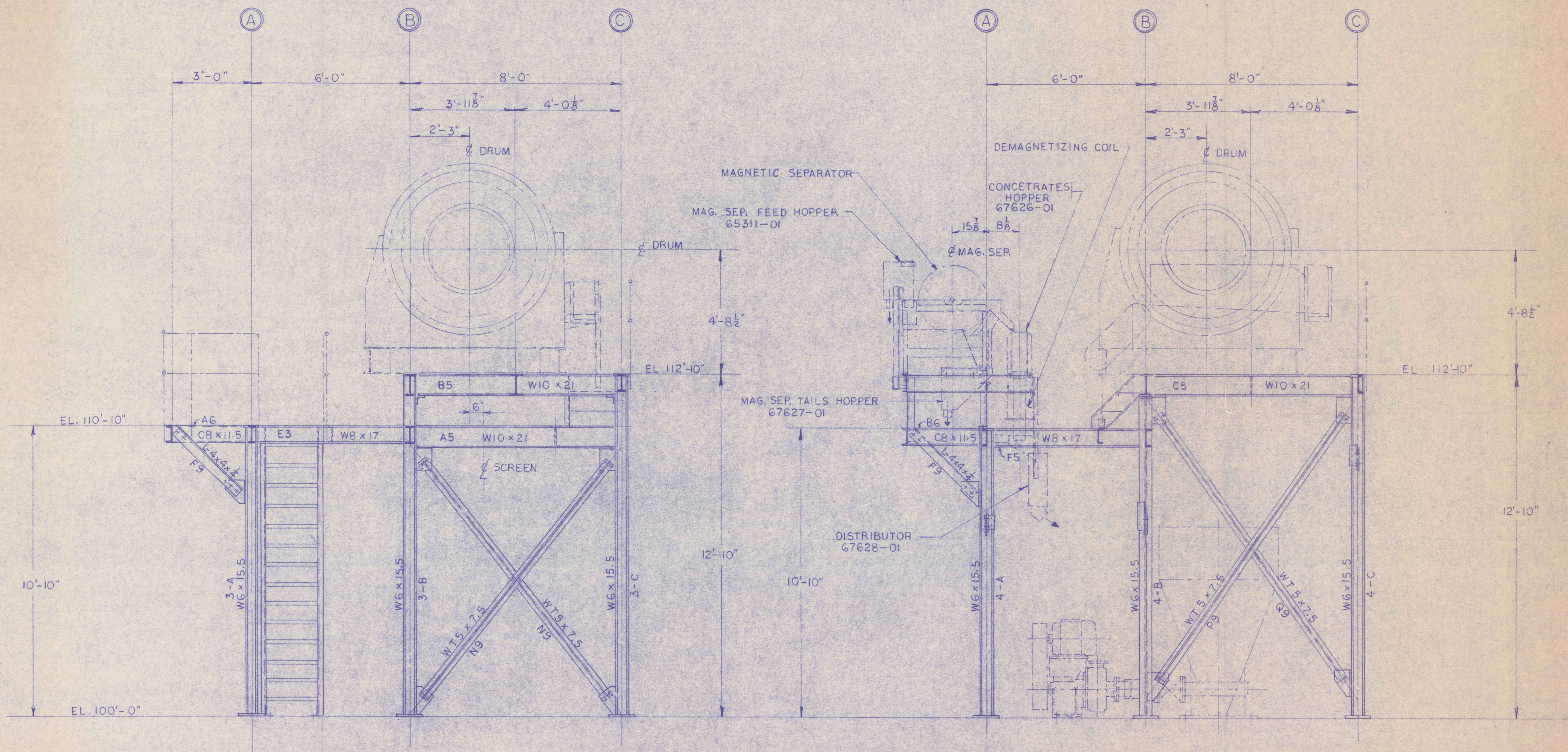
SECTION AT COL. LINE ③
