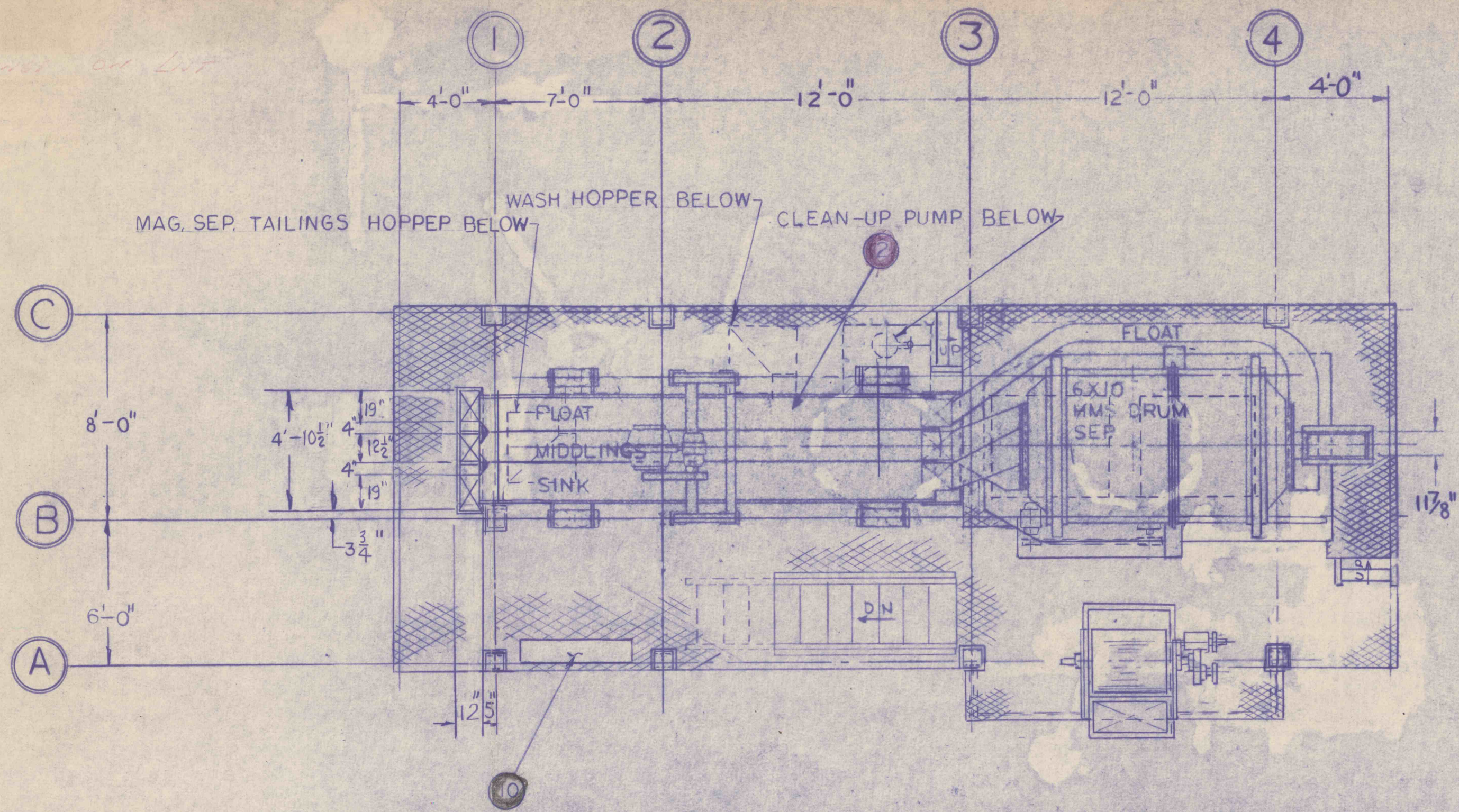
PLAN
