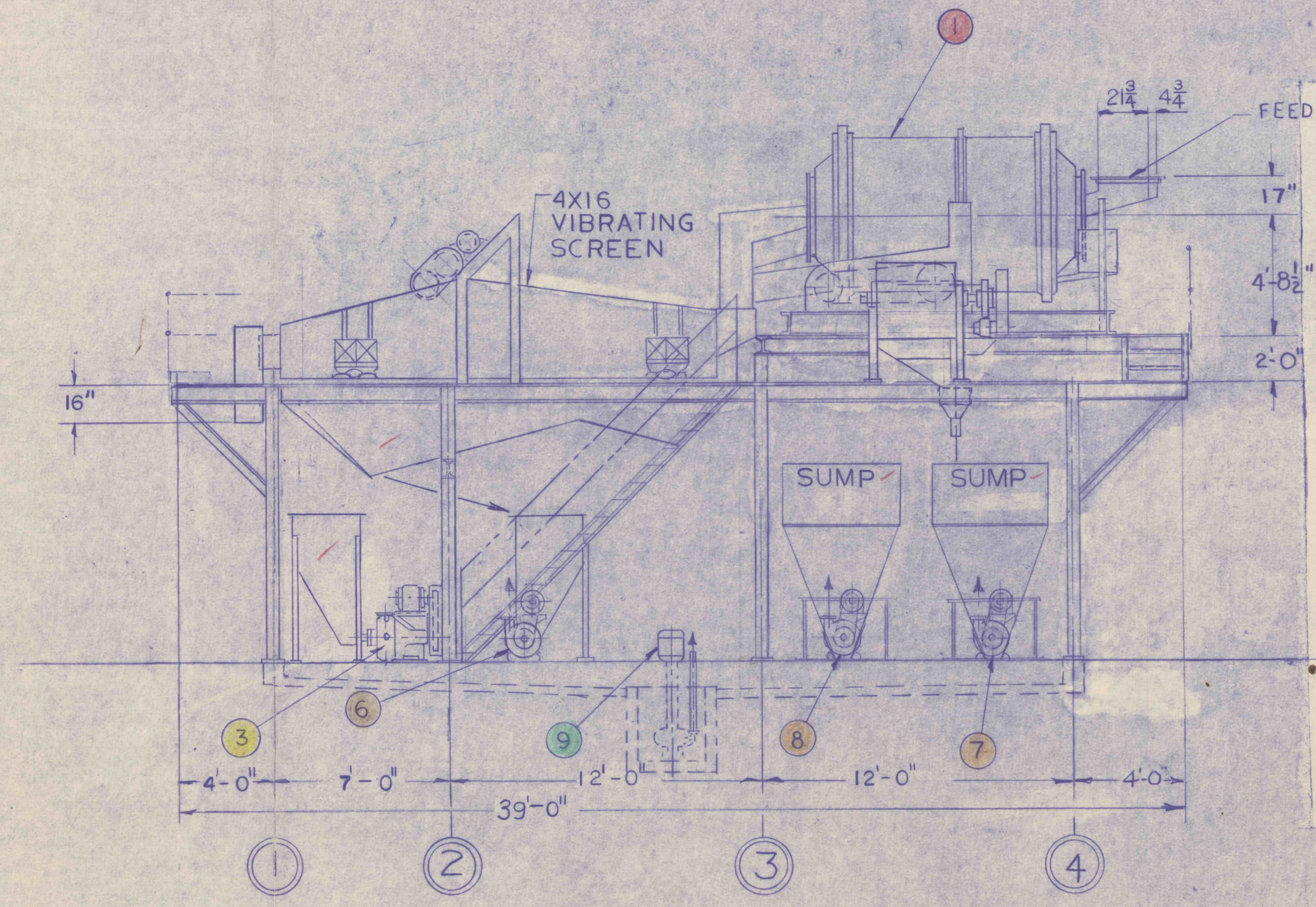
SIDE ELEVATION
