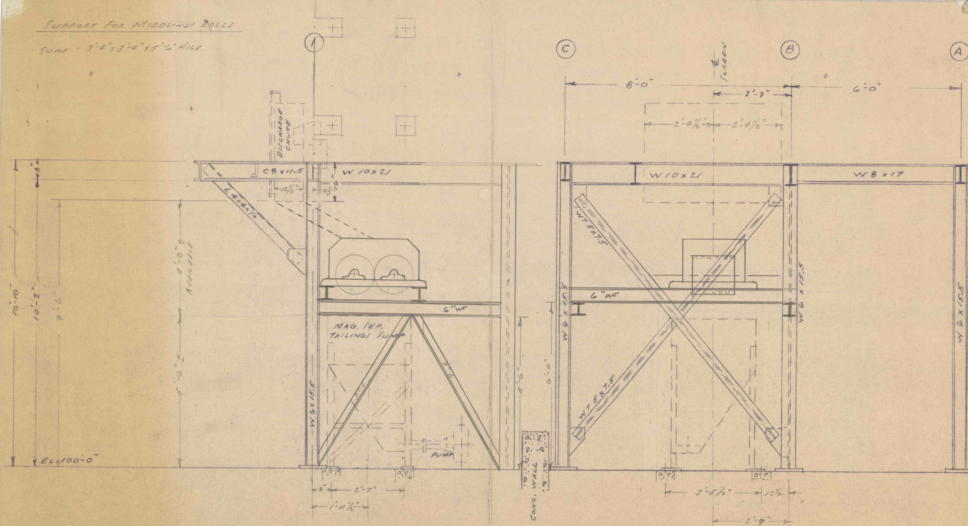
SECTION AT COL. LINE B
