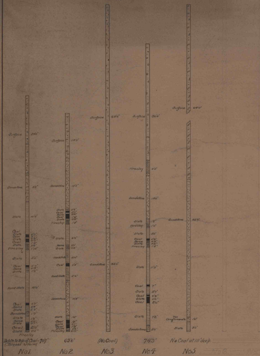
DIAMOND DRILL HOLE SECTIONS. Scale 1"=10'
