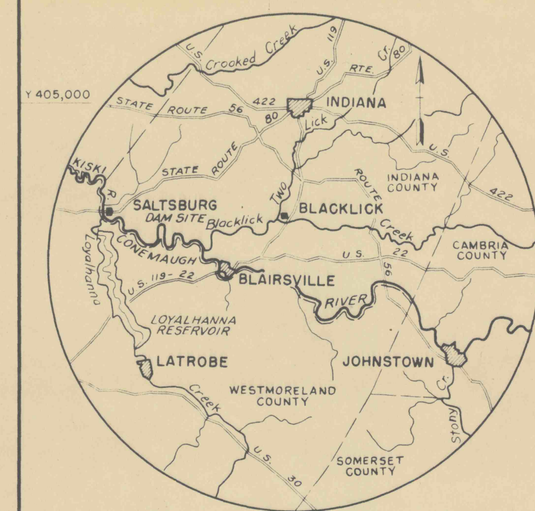
VICINITY MAP SCALE OF MILES 0 5 10 15
