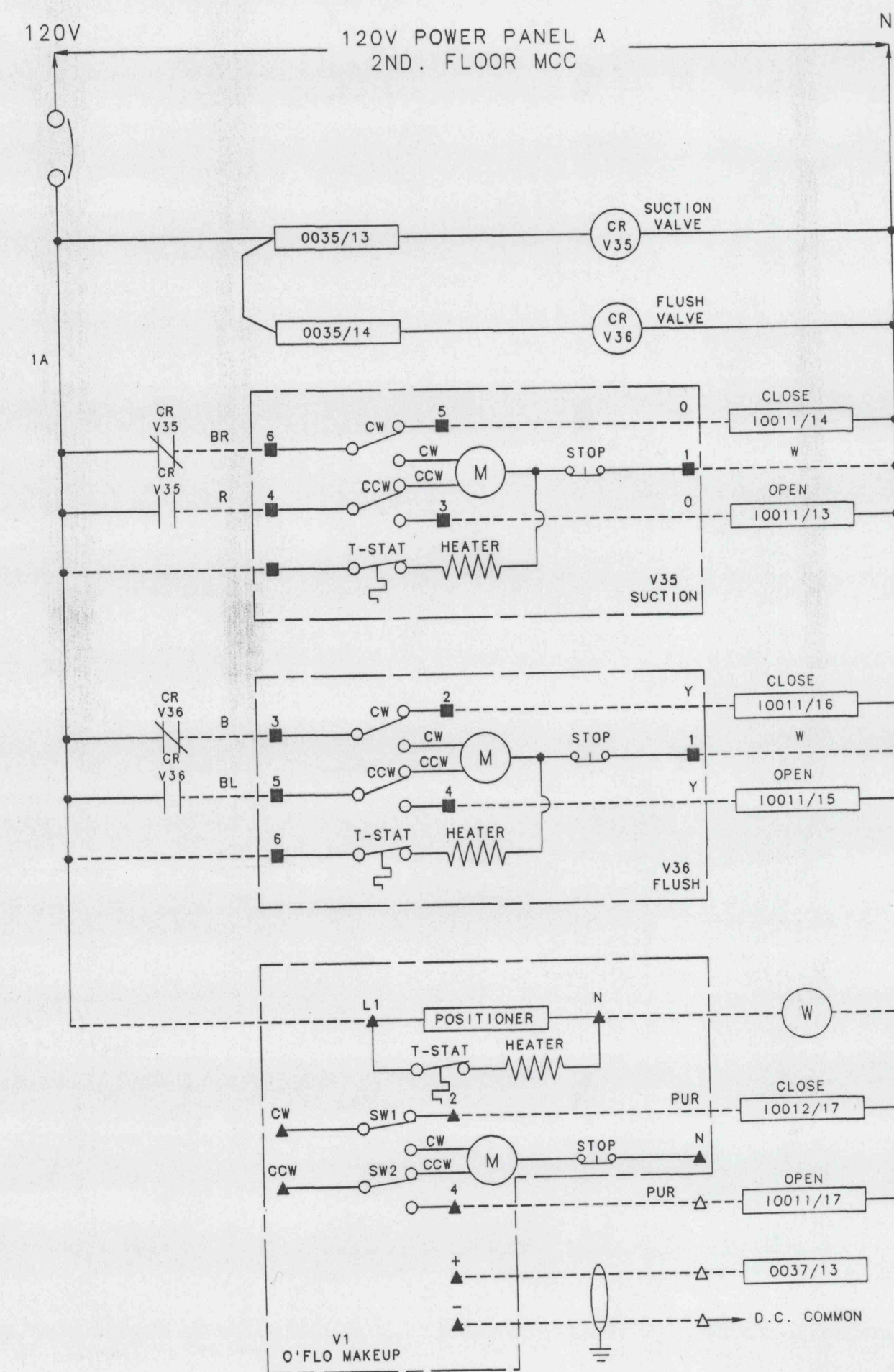
V1, V35, & V36 VALVES CIRCUIT
