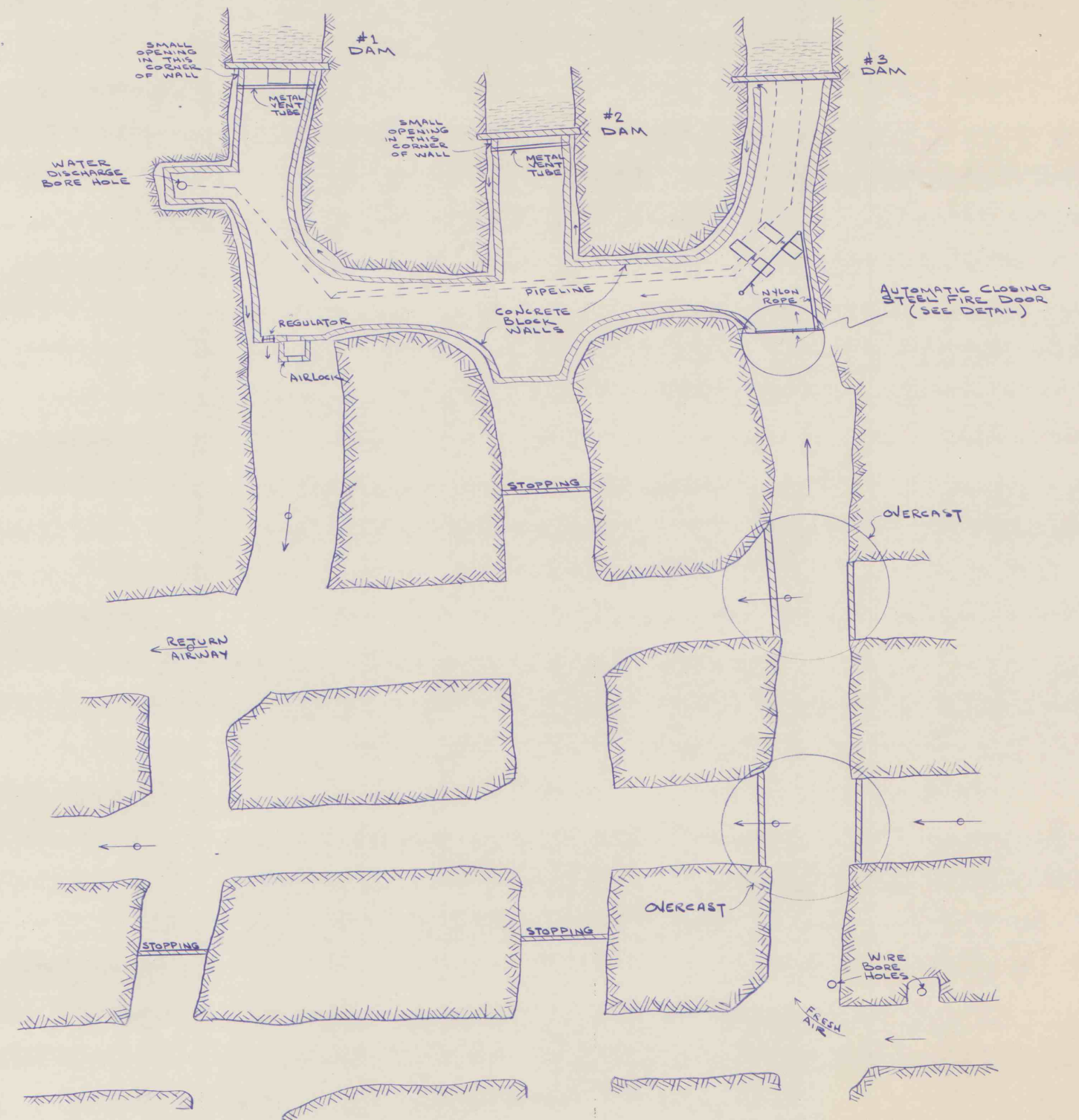
GENERAL PLAN SCALE: 1" = 10'-0"
