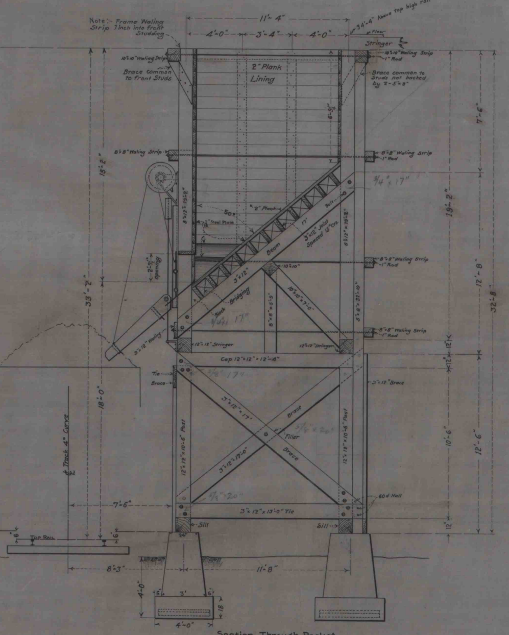
Section Through Pocket
