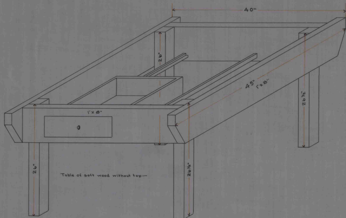
GENERAL VIEW
