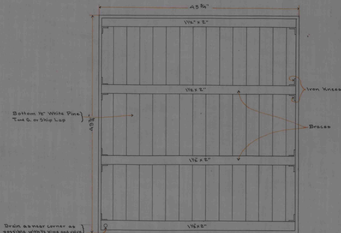
BOTTOM VIEW
