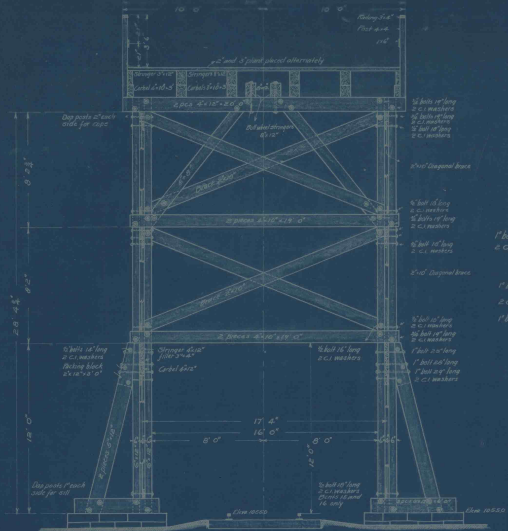
DETAILS BENT NO. 16
