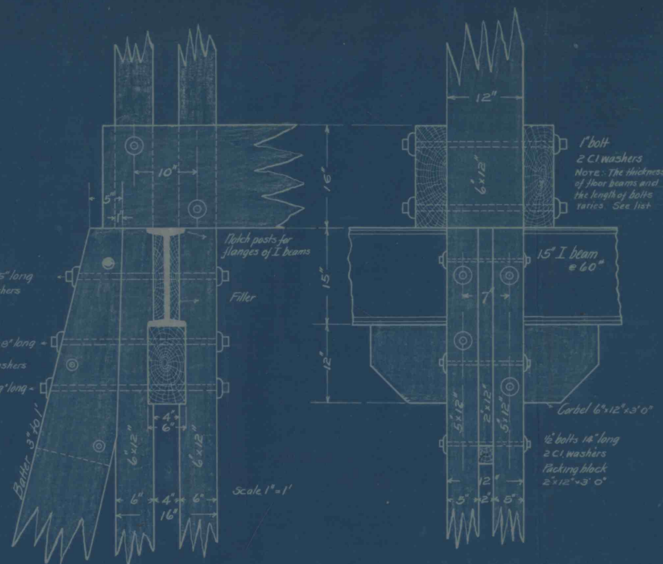
DETAILS OF BATTER POST JOINT AND FLOOR BEAM CONNECTION
