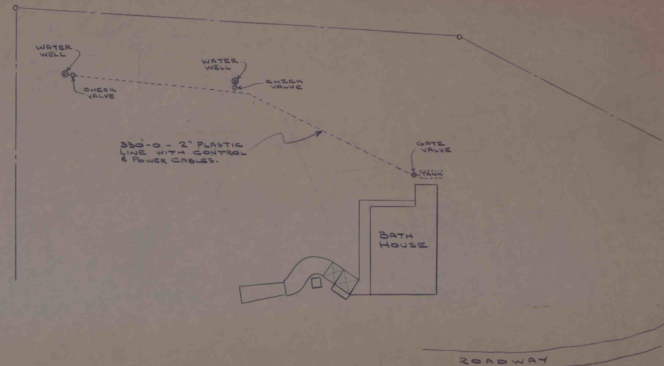
— GENERAL PLAN — SCALE: 1" = 50'-0"
