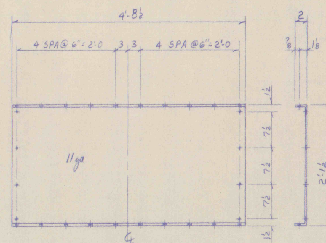
COVER R "A12" NOT REQUIRED 1-REQ'D AS SHOWN
