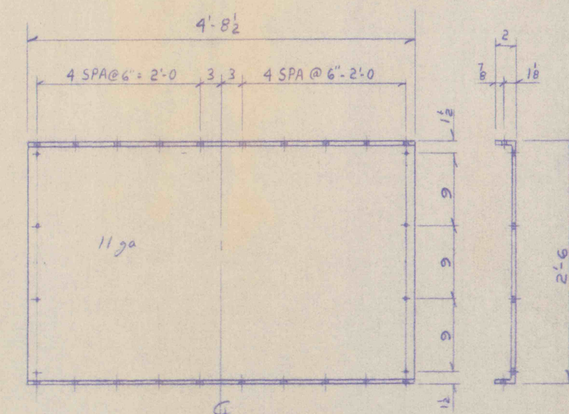
COVER R "A11" NOT REQUIRED 2-REQ'D AS SHOWN
