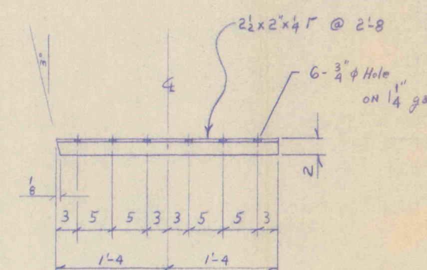
ANGLE "A9" REQUIRED 2-REQ'D 1-AS SHOWN 1-OPP. HAND
