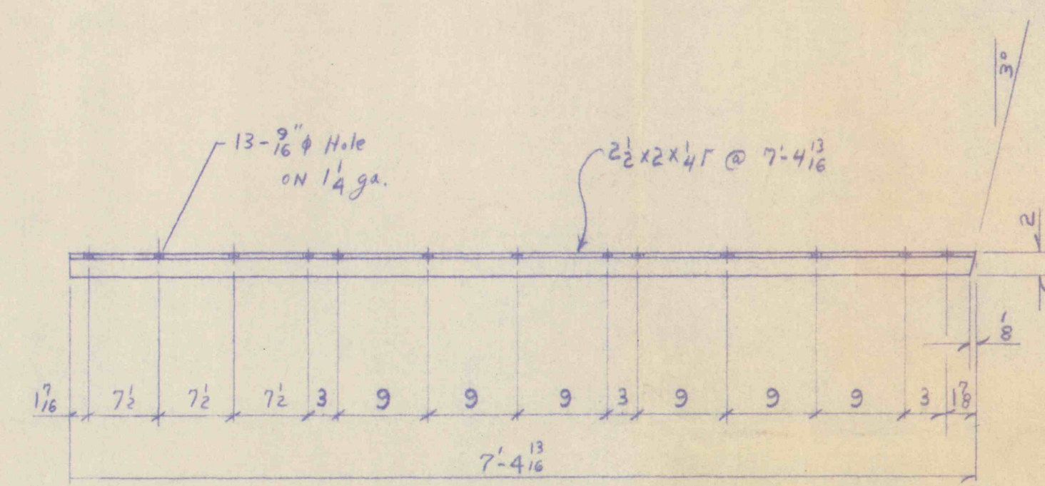
ANGLE "A10" REQUIRED 2-REQ'D 1-AS SHOWN 1-OPP. HAND
