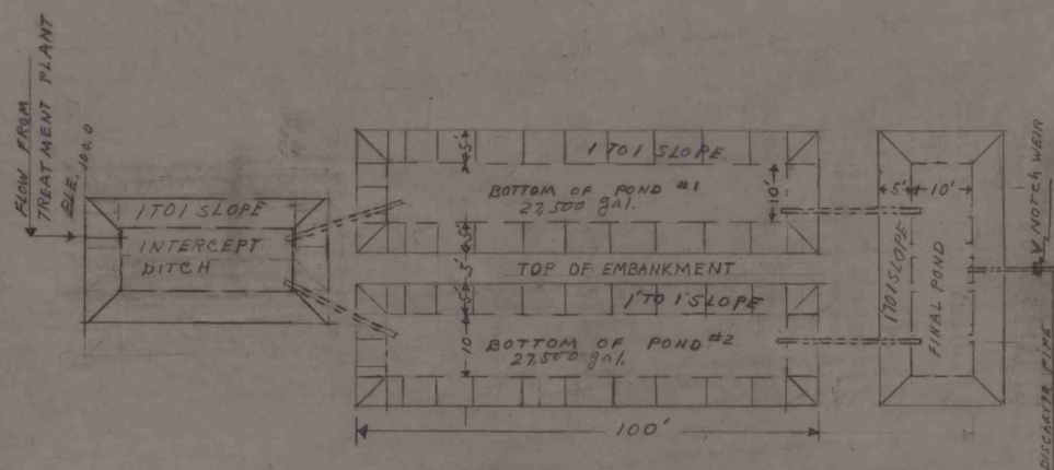
SEDIMENT BASINS TOP VIEW
