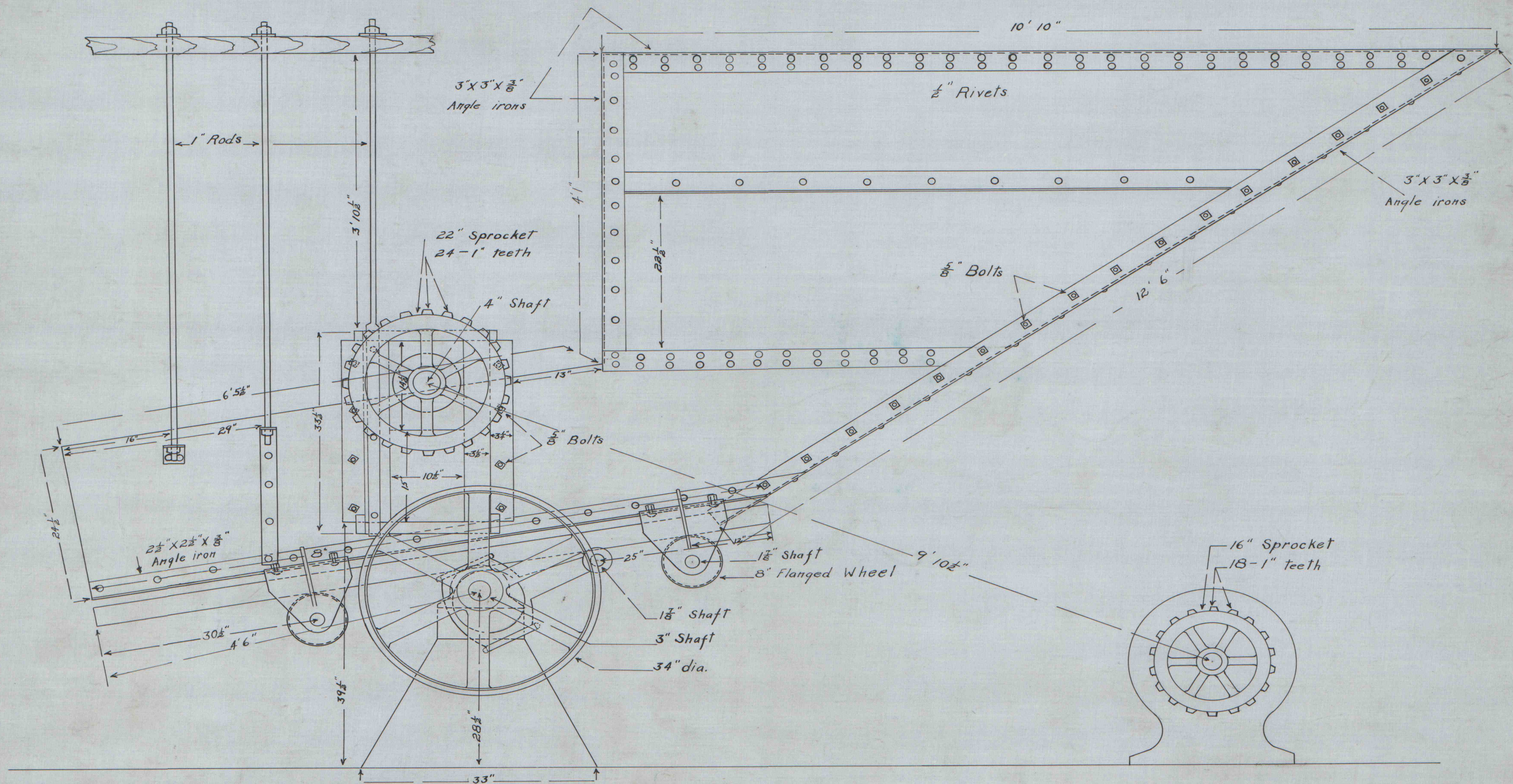
SIDE VIEW PROCTOR NO.1 CRUSHER INSTALLATION. 9/15/39 N. A.
