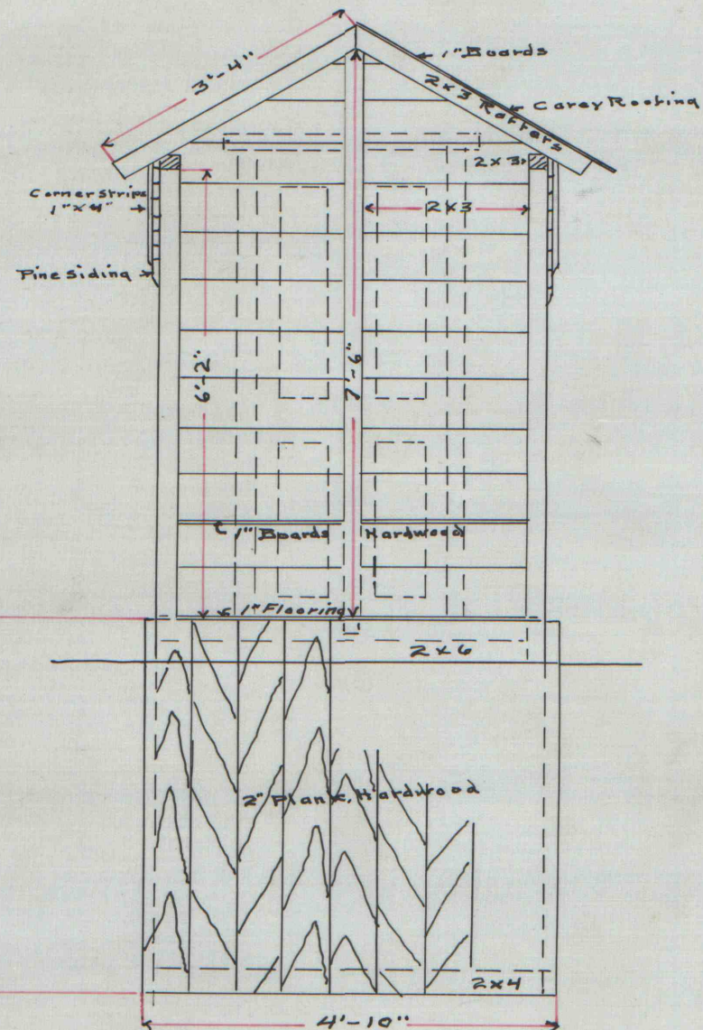
Front Elev.
