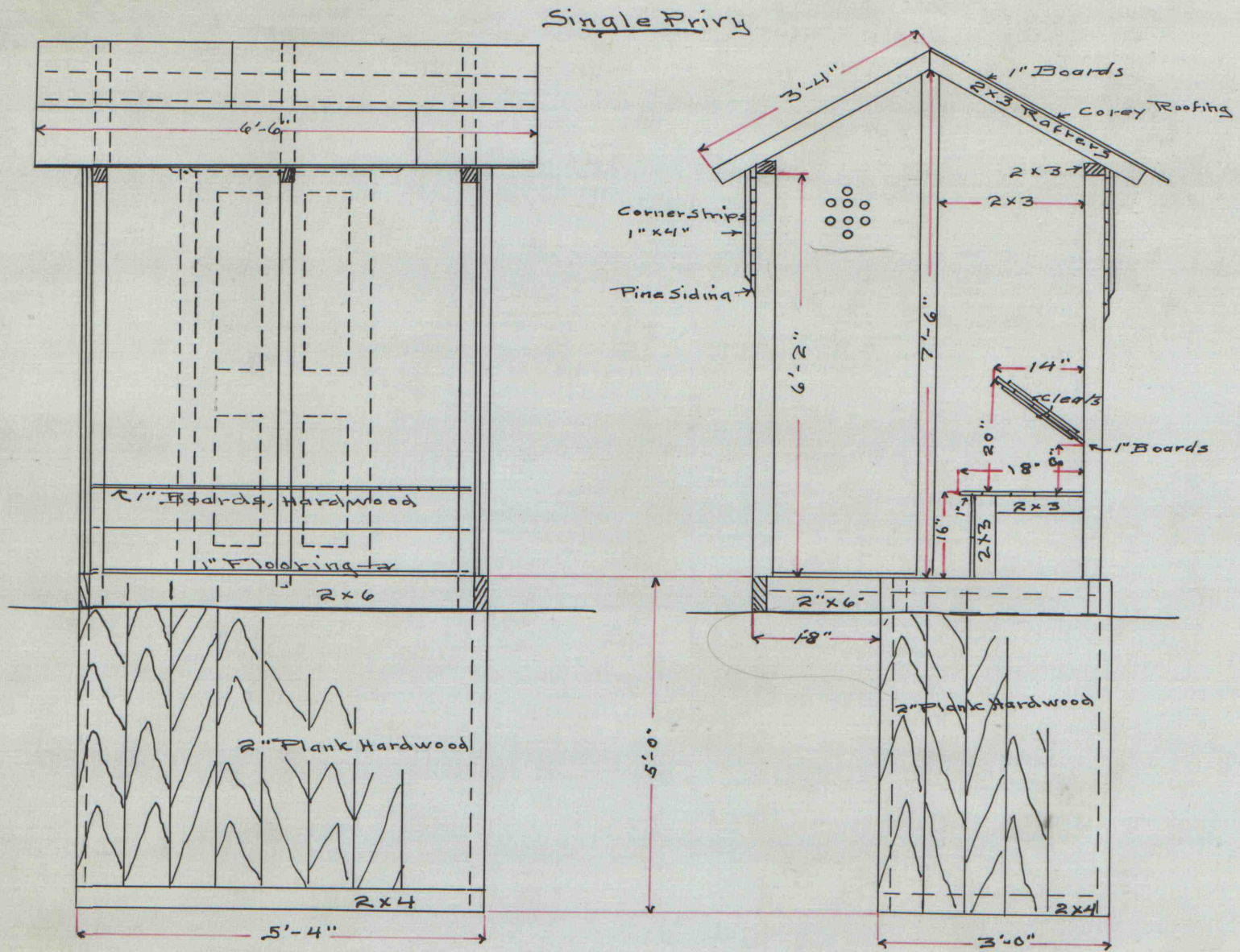
Front Elev.
