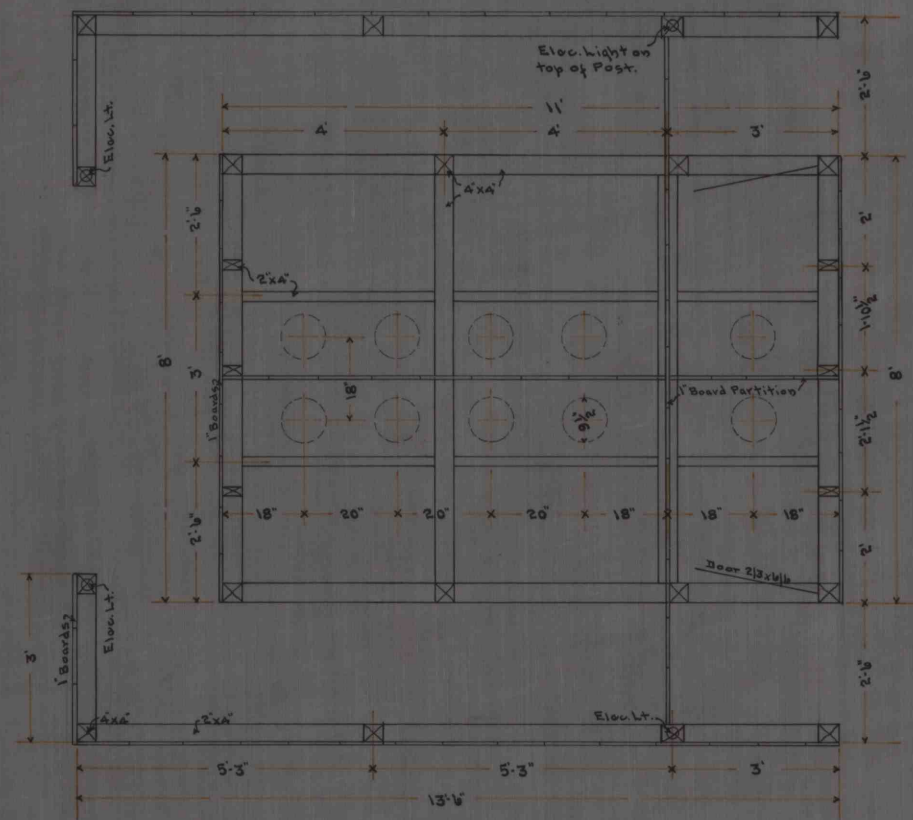
— Plan of Building and Fence —
