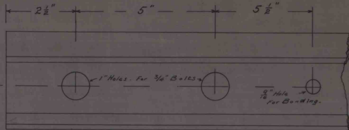
Angle Bar 20"
