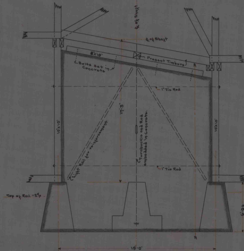
Elevation at Bents 12 and 13 showing Present Concrete Footings and Proposed Concrete Walls.
