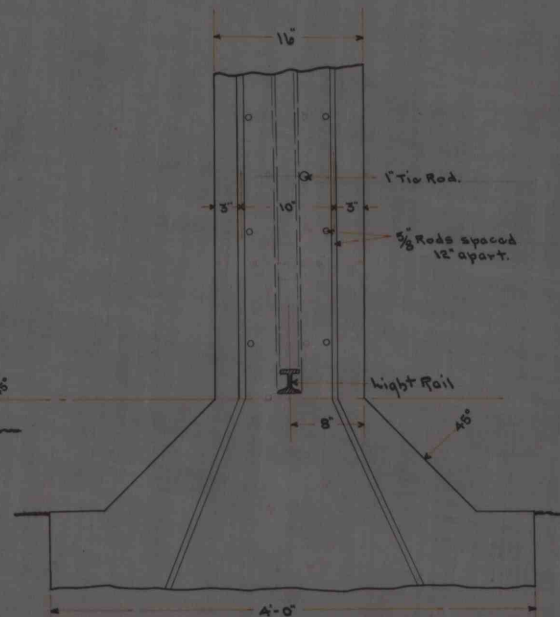
Cross Section of Walls Showing Reinforcement Plan.
