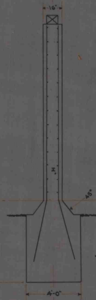
Cross Section Thru A-A
