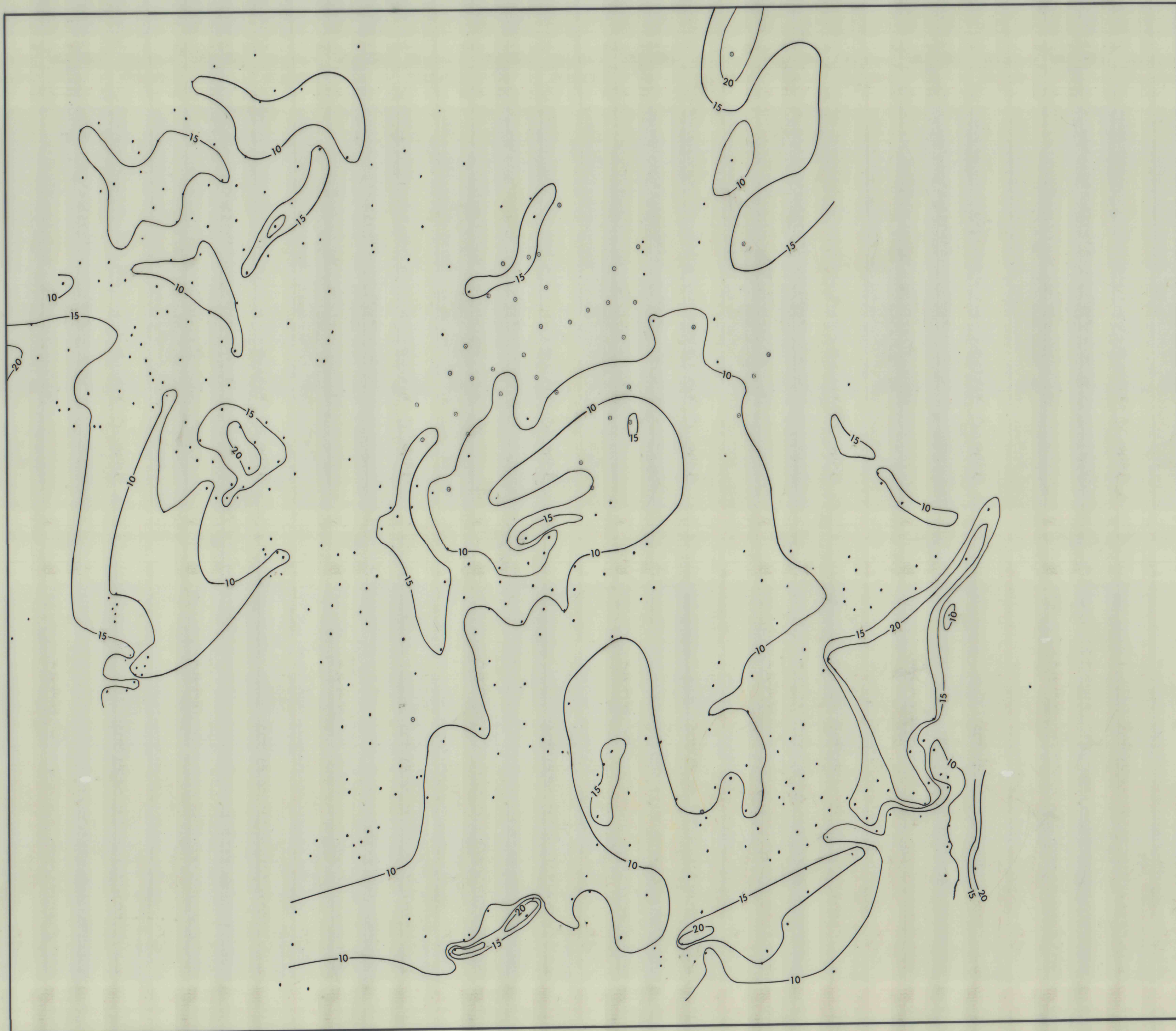
ISO-ASH MAP OF LOWER BENCH OF UPPER FREEPORT COAL
