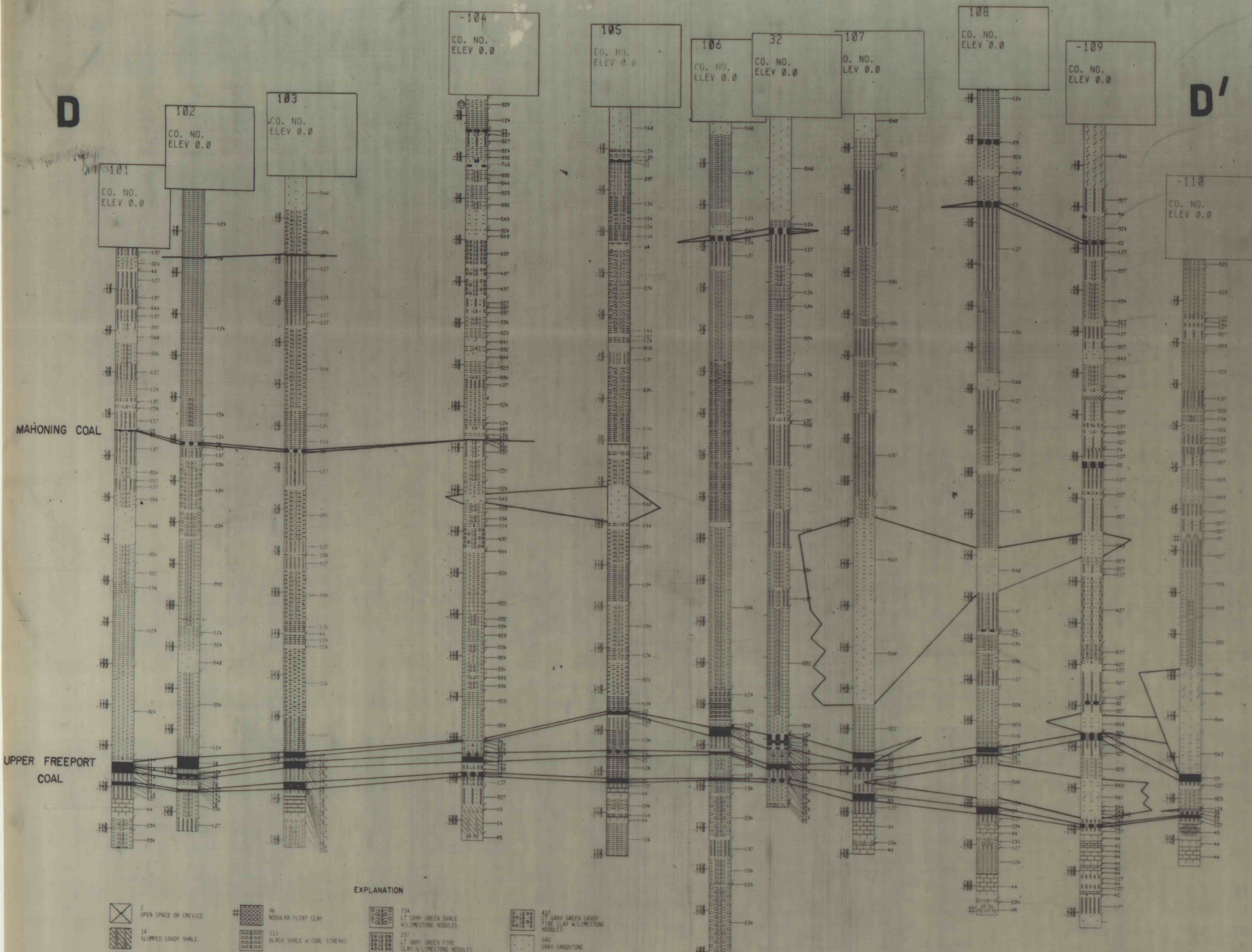
PLATE 5 CROSS SECTION D-D'
