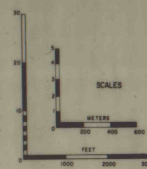
PLATE 8 CROSS SECTION E-E'
