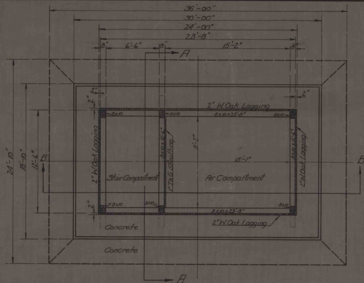
Plan Of Top Of Shaft
