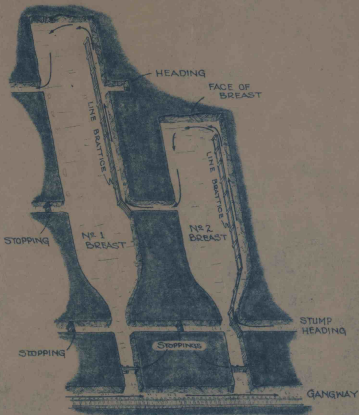
VENTILATION OF BREASTS IN FLAT OR LIGHT PITCHING SEAMS
