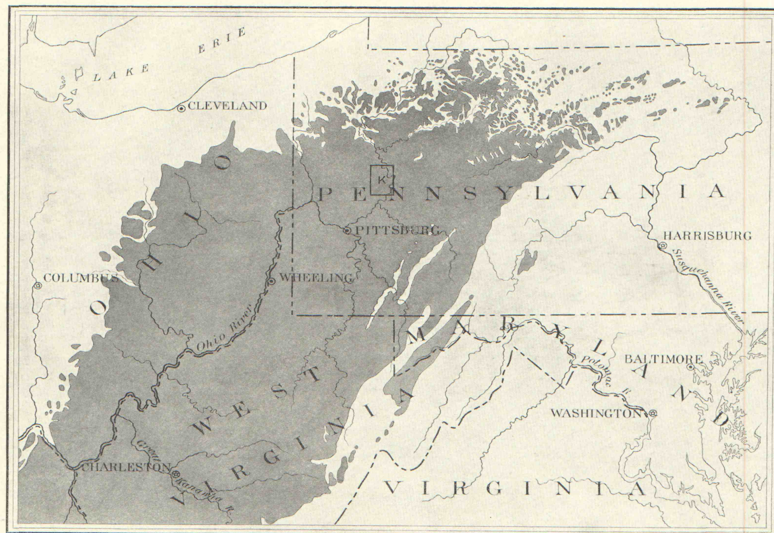
FIG. 11.—MAP SHOWING THE EXTENT OF THE NORTHERN PART OF THE APPALACHIAN COAL FIELD. The position of the Kittanning quadrangle within the coal field is shown by the rectangle.
