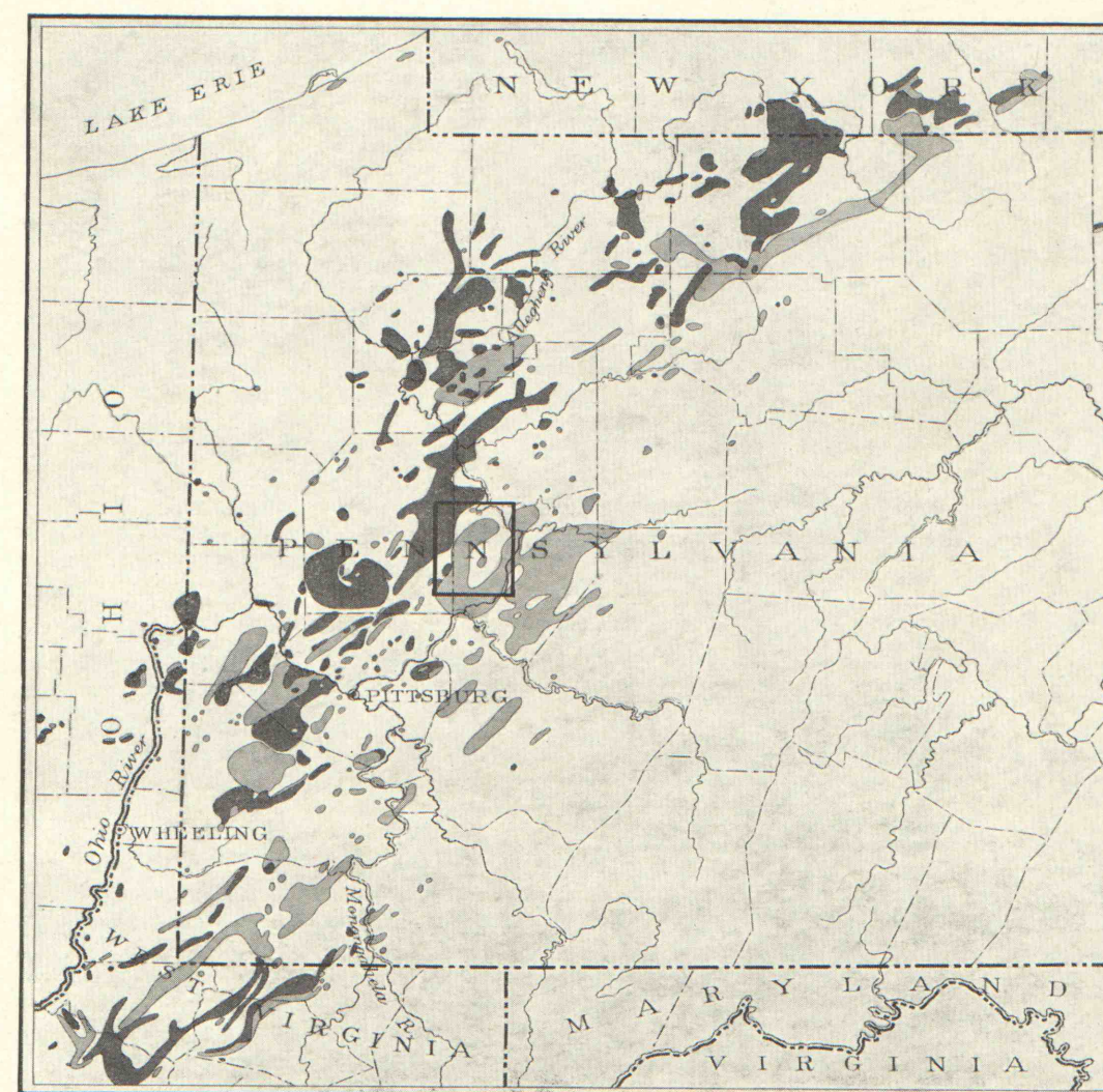
FIG. 12.—MAP OF THE OIL AND GAS PRODUCING AREAS OF THE NORTHERN APPALACHIANS. Compiled from map by the Second Geological Survey of Pennsylvania, and from maps by the United States Geological Survey. Dark areas, oil; lighter areas, gas. The location of the Kittanning quadrangle is shown by the rectangle.
