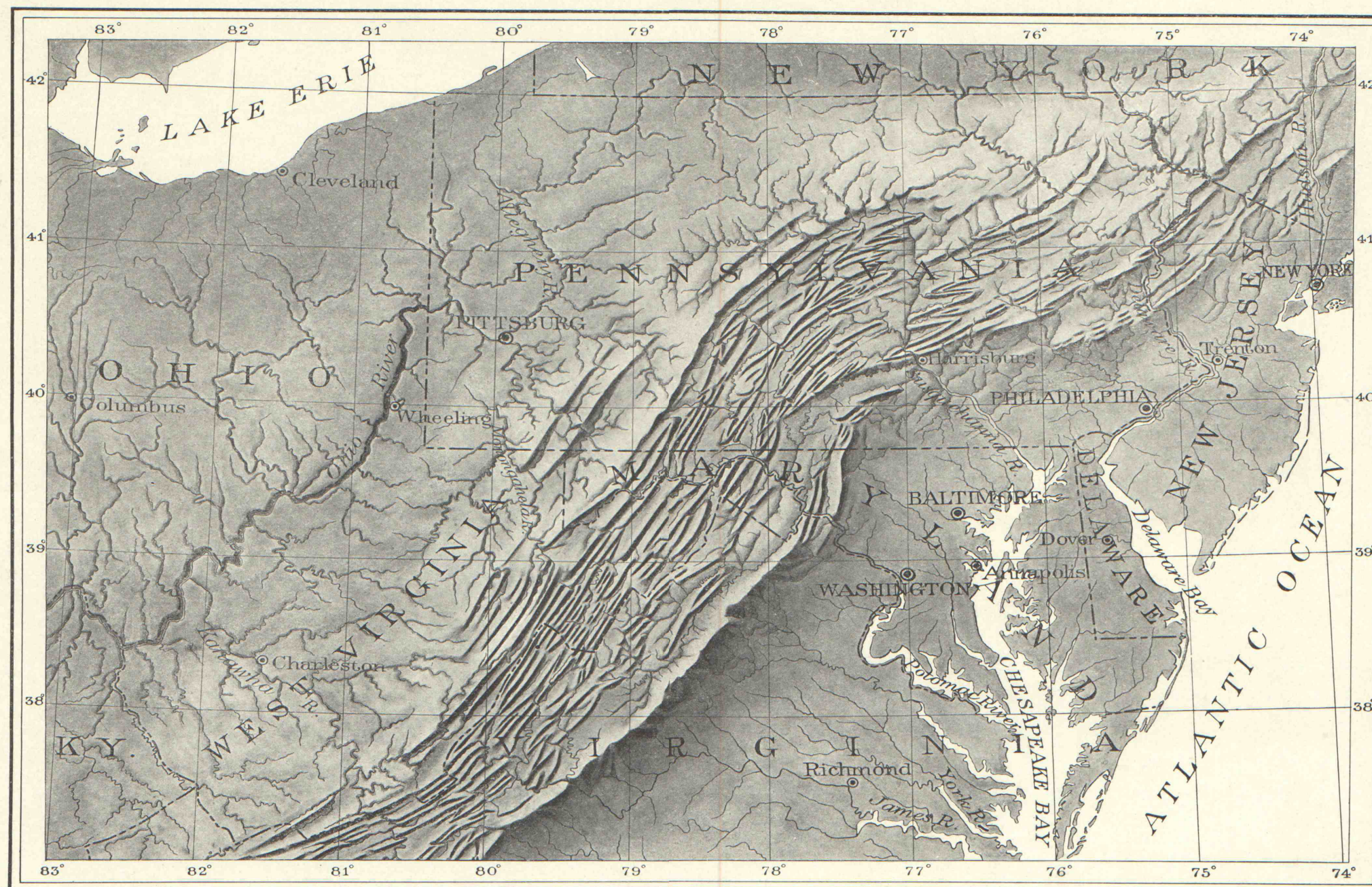
FIG. 10.—RELIEF MAP OF THE NORTHERN APPALACHIAN MOUNTAINS. The Kittanning quadrangle is situated on the plateau lying west of the belt of valley ridges, in the west-central part of Pennsylvania.
