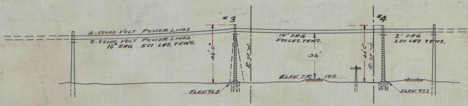
PROFILE
