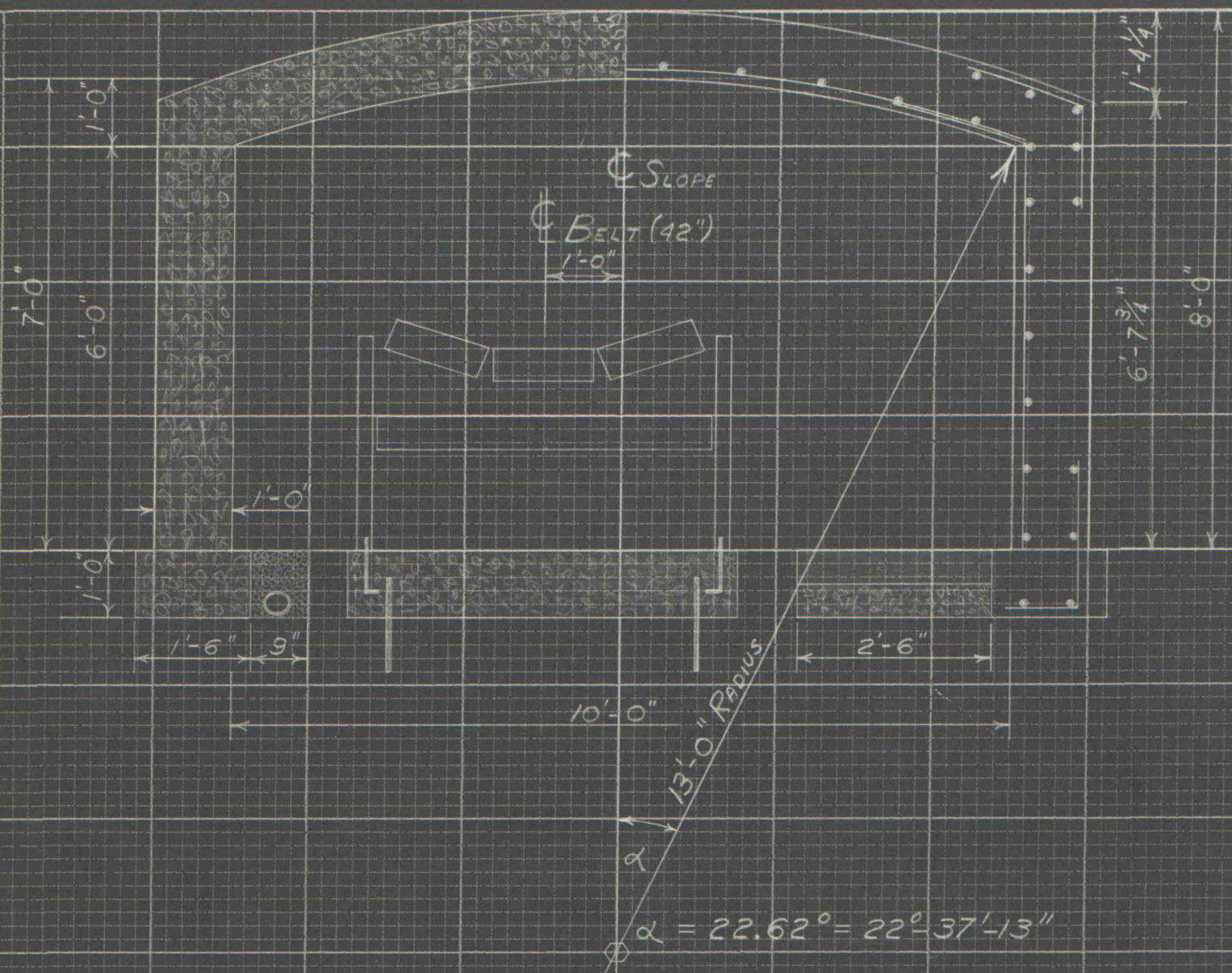
7' x 10' BELT SLOPE
