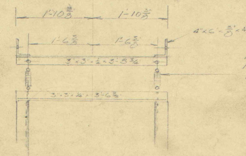
SECTION X-X1
