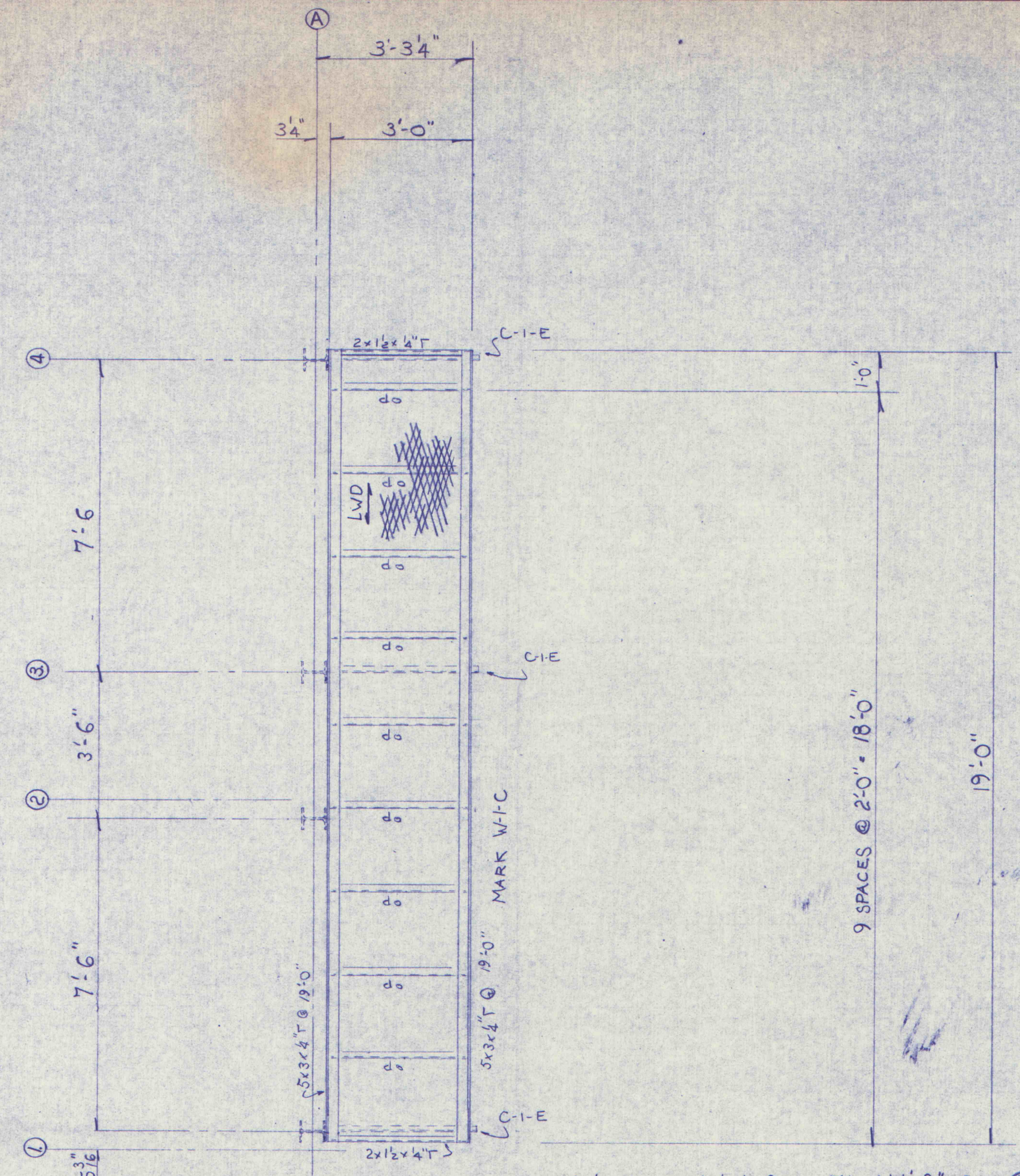
WALKWAY W-1-C @ EL 111'-3" COL A W-1-C @ EL 123'-1 1/2" COL A 2 REQ'D AS SHOWN
