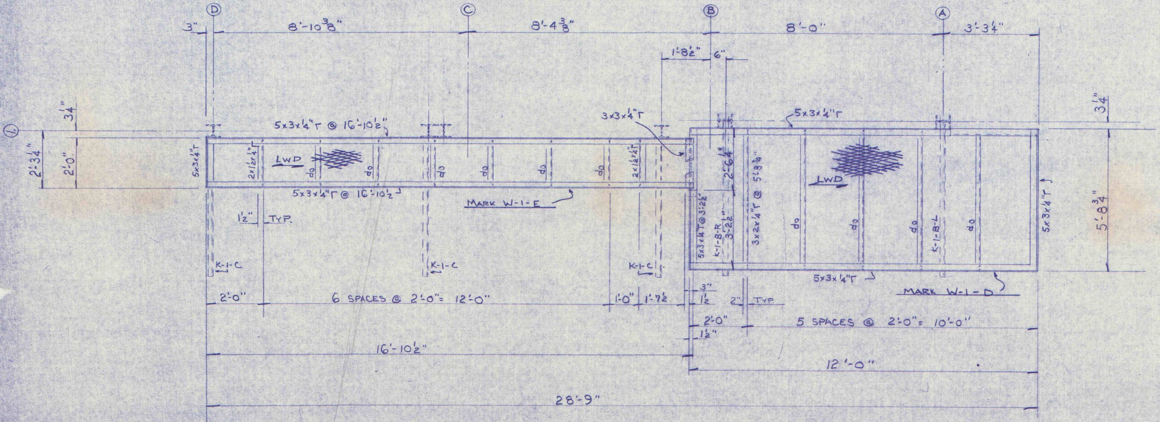
WALKWAY W-1-D & W-1-E @ EL 111'-3" COL 1
