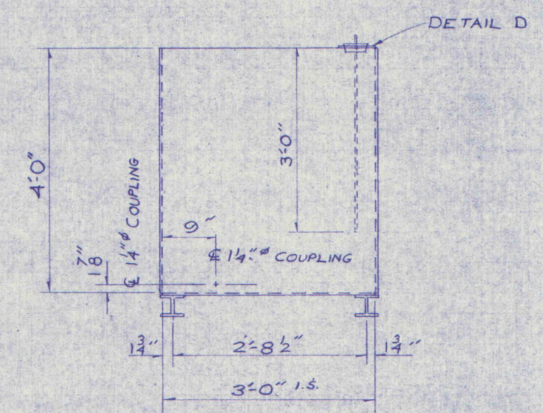
GLAND SEAL TANK DETAIL C-C SCALE 3/4"=1'-0"
