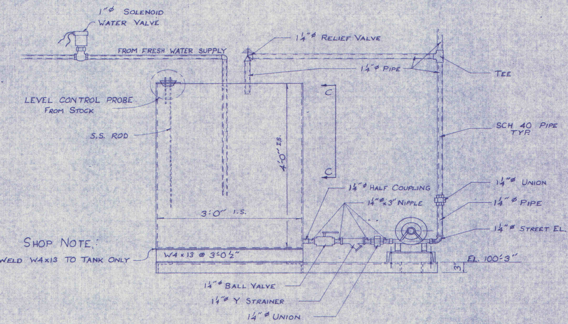
GLAND SEAL PUMP SUCTION PIPING DETAILS DETAIL A-A 1"=1'-0"
