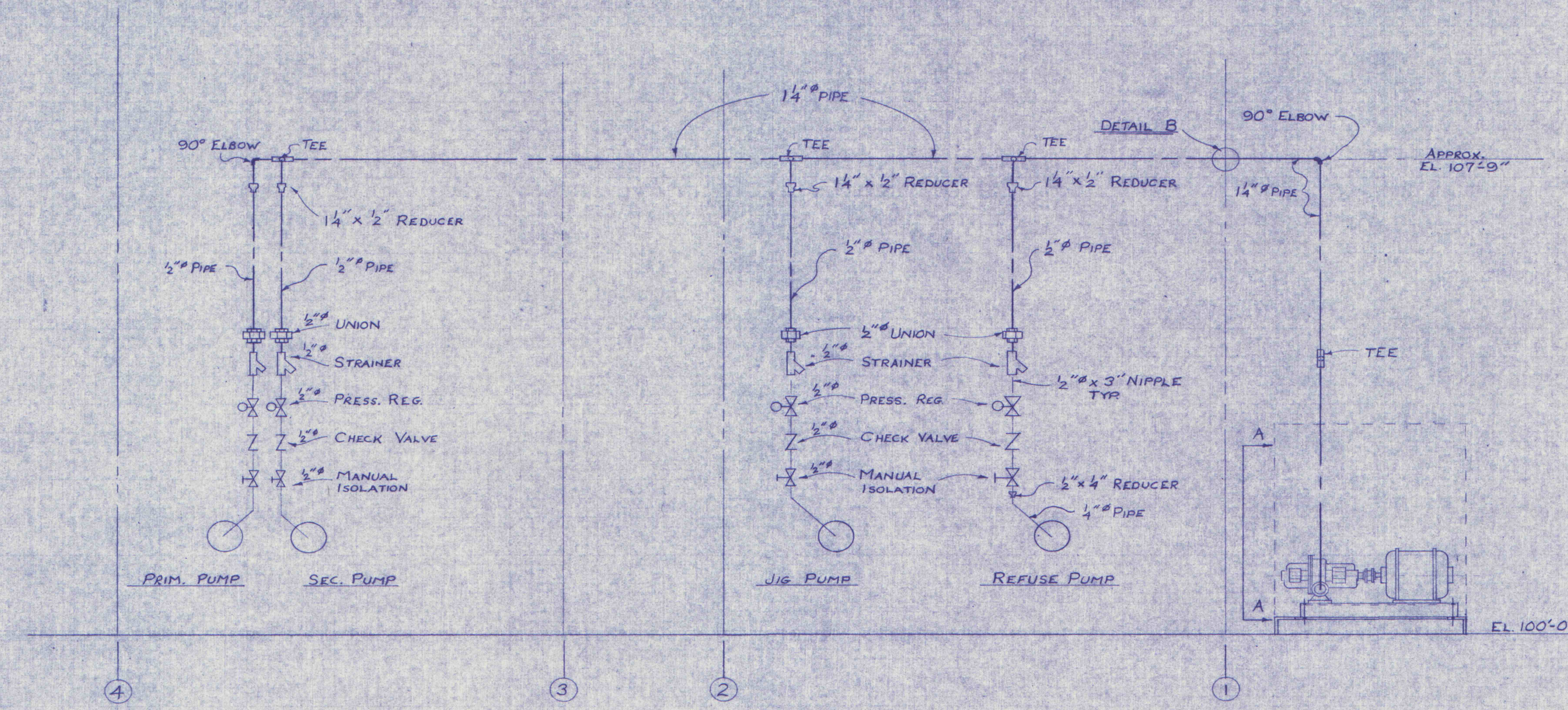
GLAND SEAL SYSTEM SCHEMATIC SCALE - NONE
