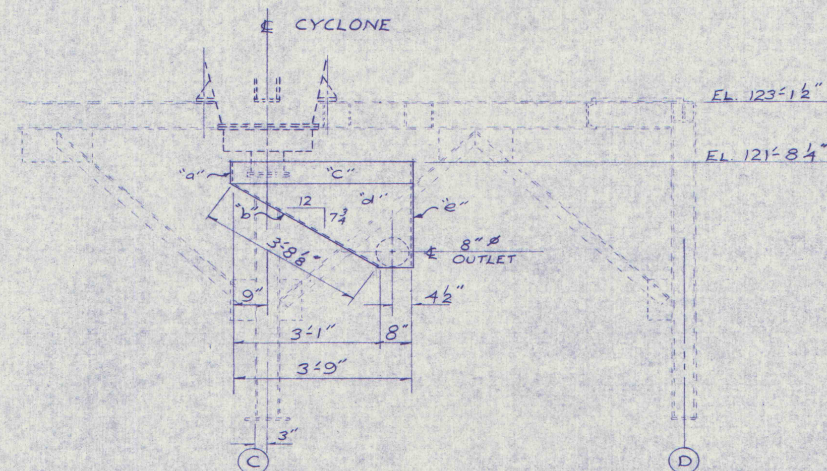
SECONDARY CYCLONE UNDERFLOW SUMP
