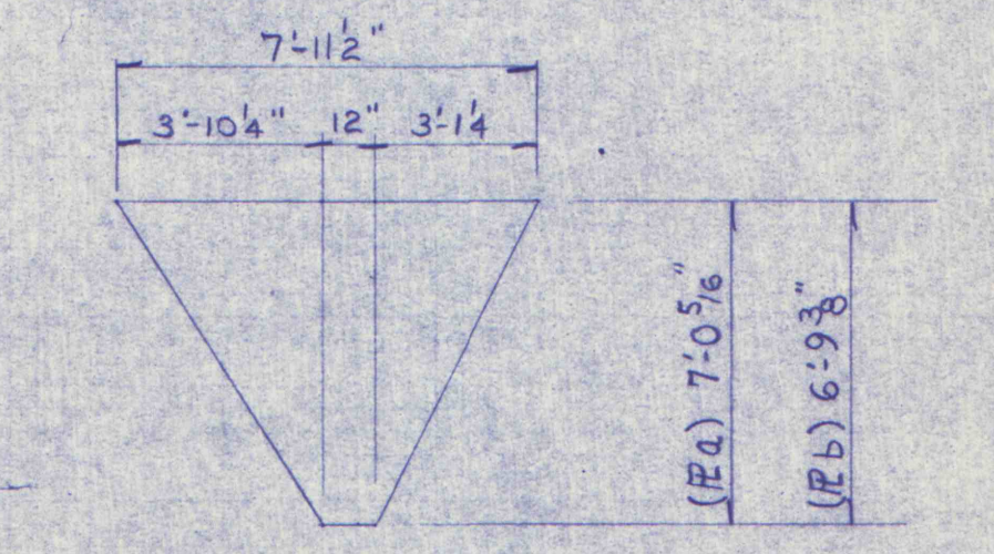
PA 1 REQ'D. PER SUMP PB 1 REQ'D. PER SUMP
