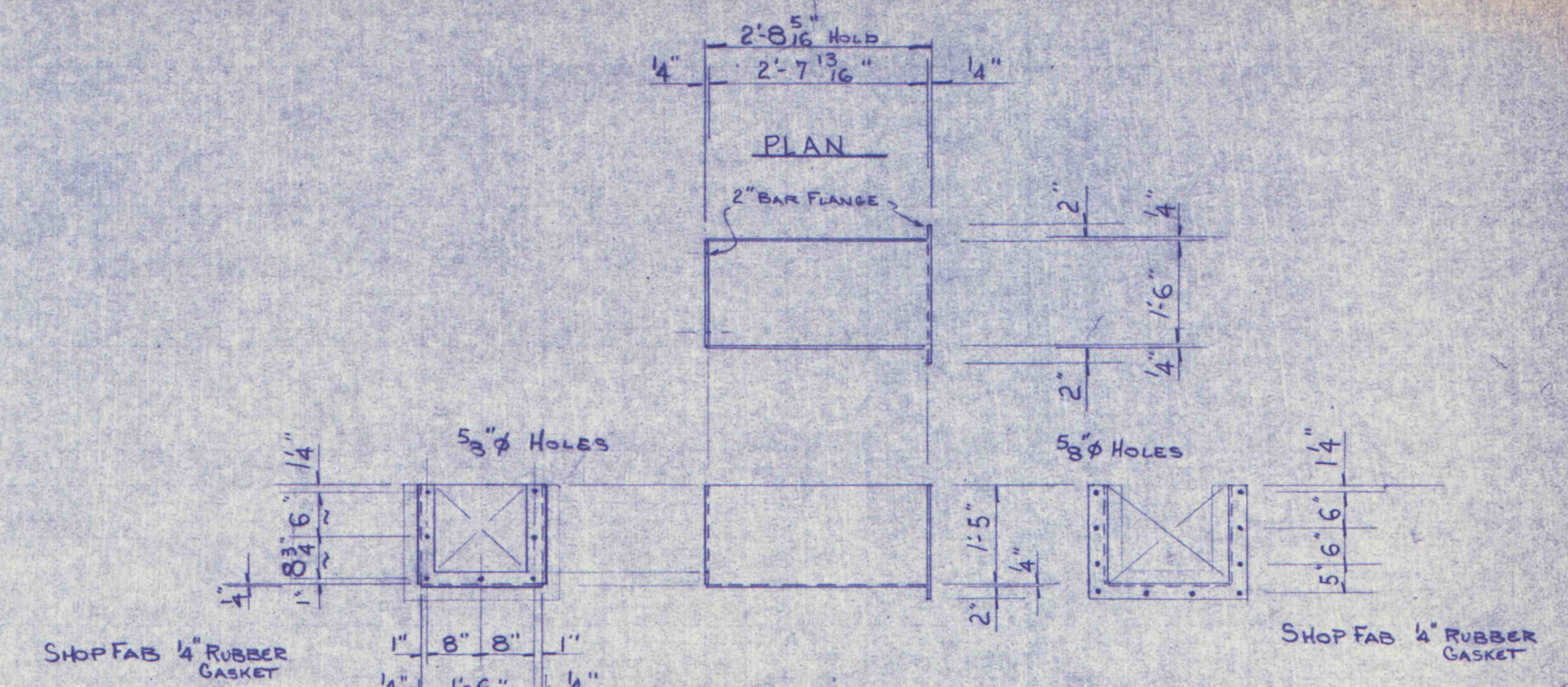
OVER FLOW LAUNDER SECONDARY SUMP TO REFUSE SUMP
