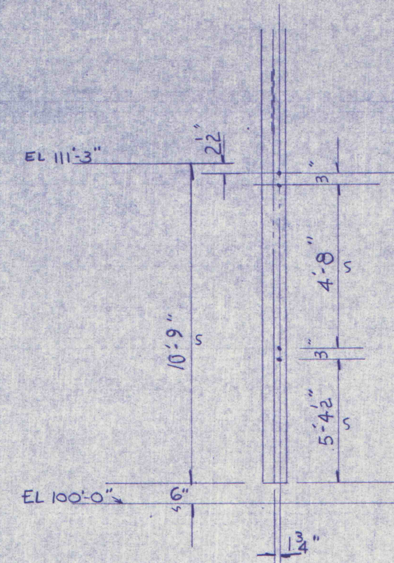
SECTION AA
