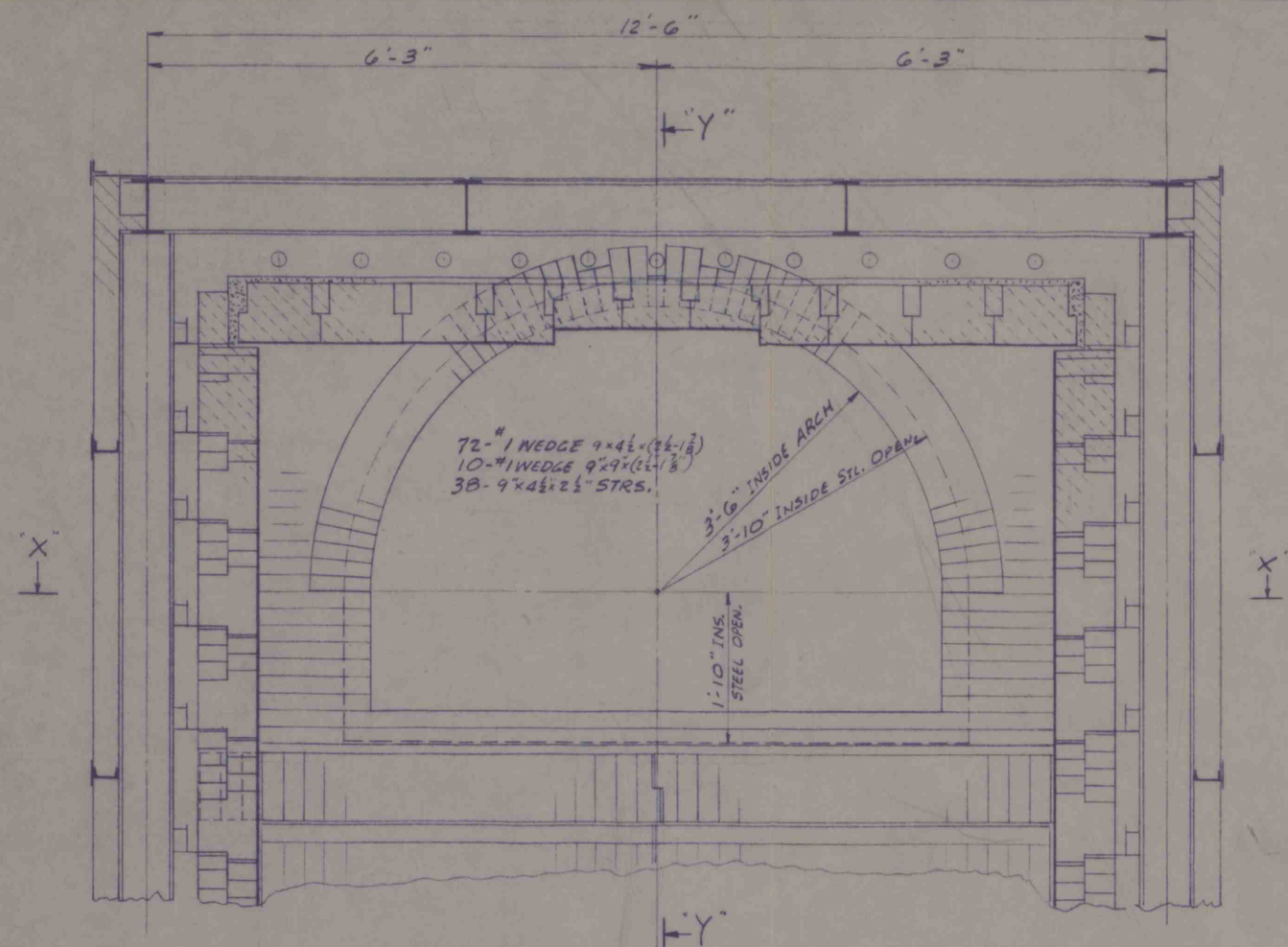
INSIDE ELEVATION CURTAIN WALL
