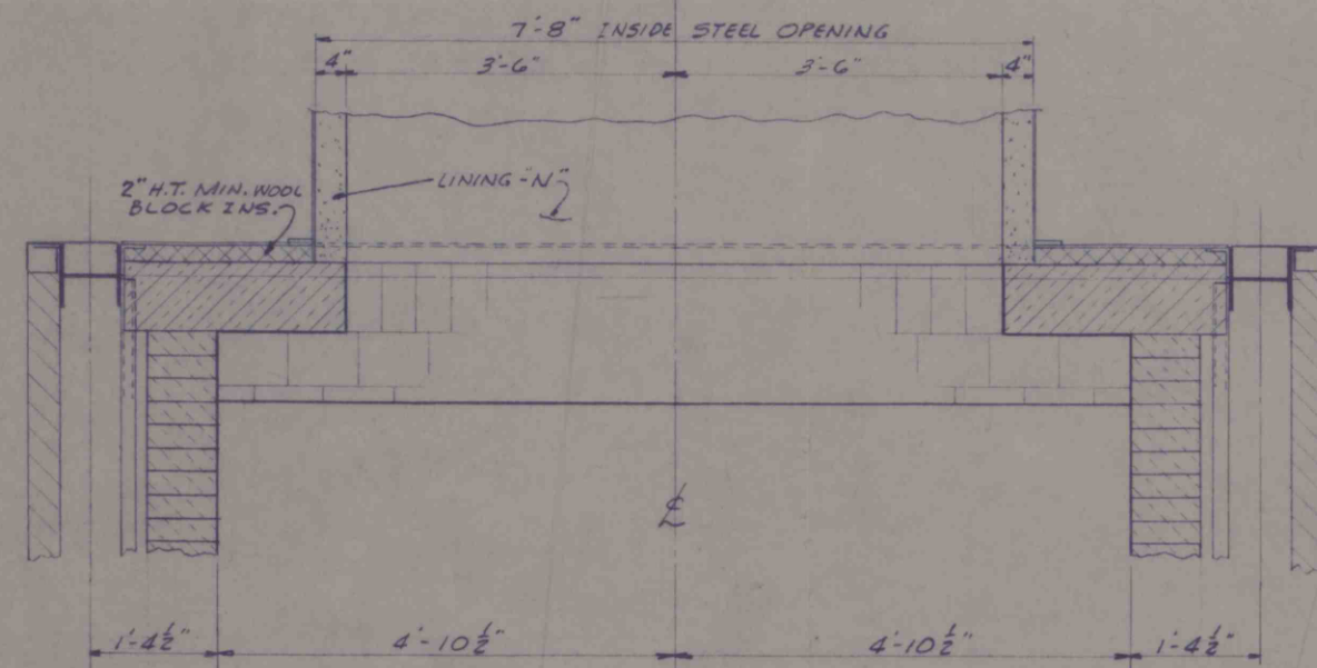
PLAN SECTION "X-X"
