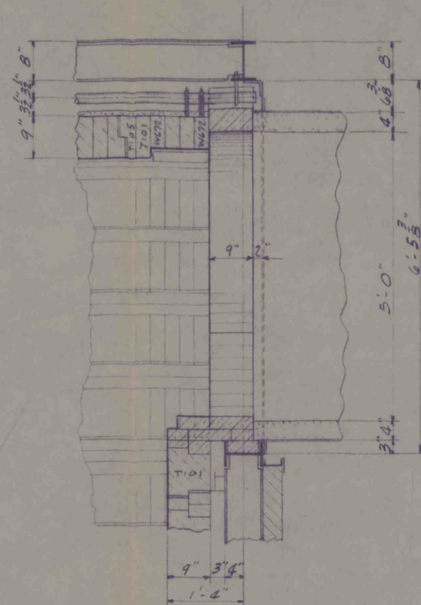
SECTION "Y-Y"
