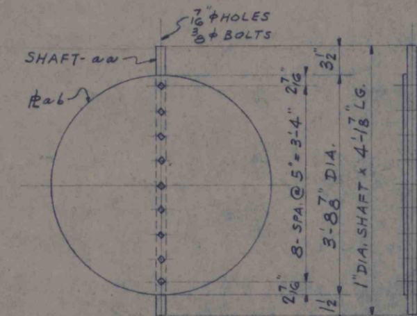
ONE (1) DAMPER MK. 11-6 ASSEMBLE WITH MK. 11-4
