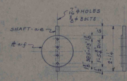
ONE (1) DAMPER MK. 11-8 ASSEMBLE WITH MK. 7-1
