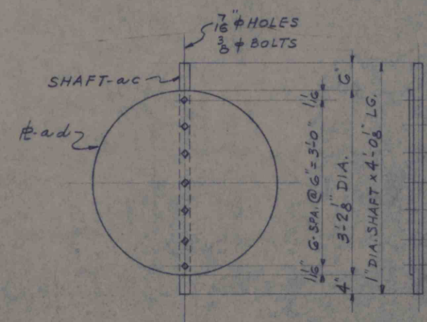
ONE (1) DAMPER MK. 11-7 ASSEMBLE WITH MK. 7-1
