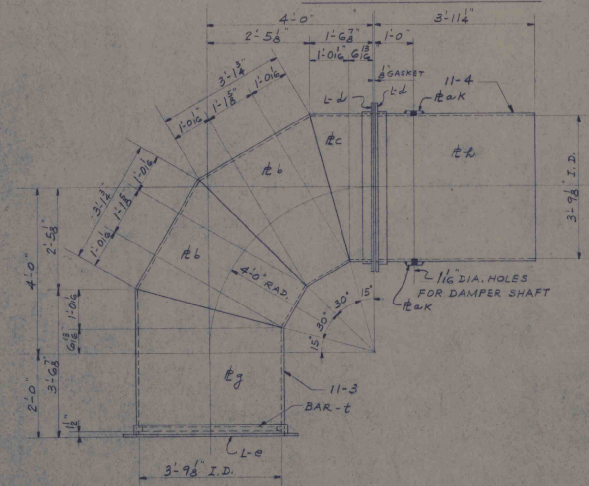
ONE (1) DUCT MK. 11-3 ONE (1) DUCT MK. 11-4
