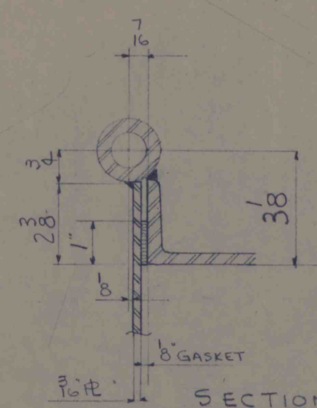
HINGE DETAIL
