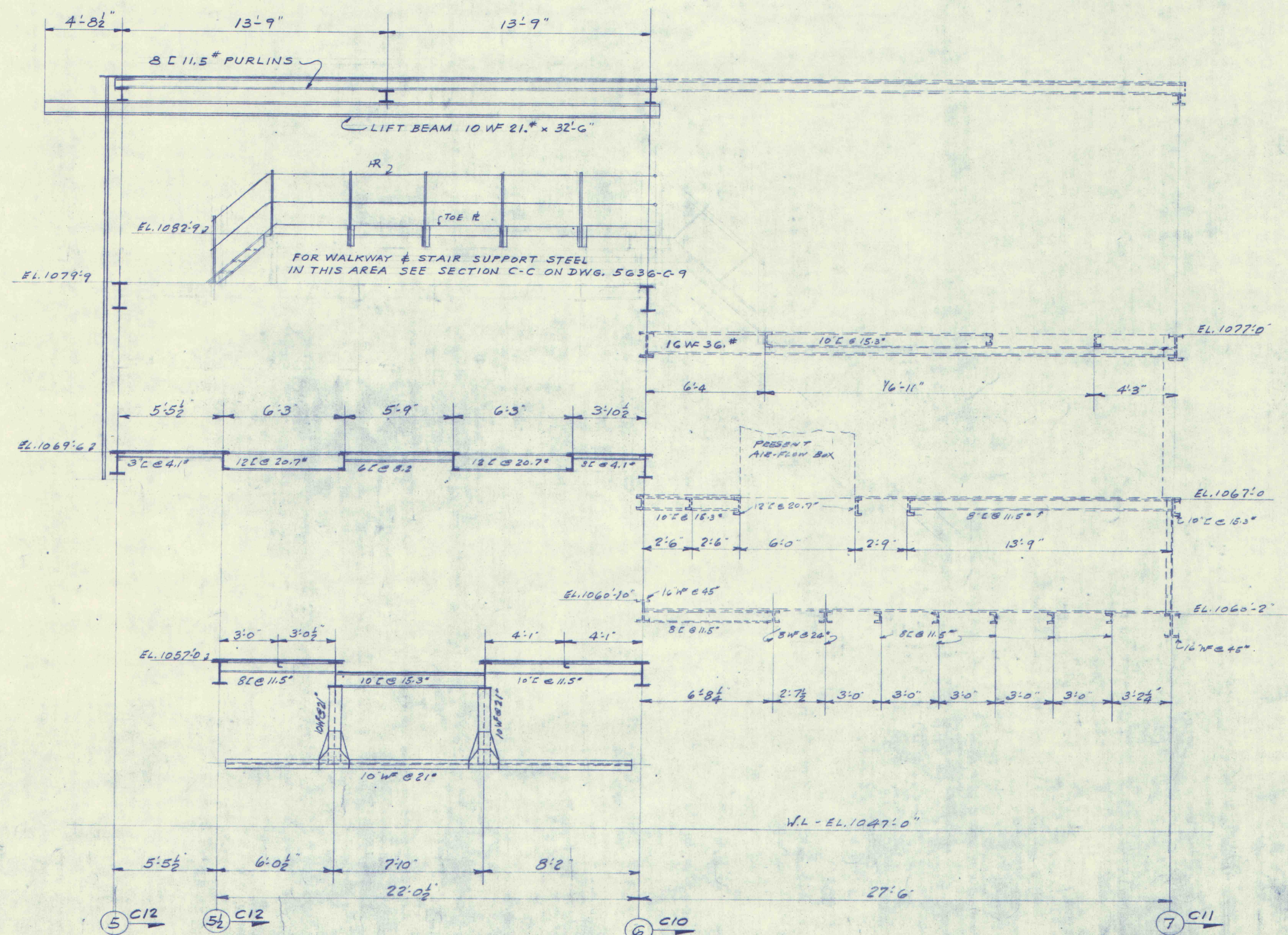
SECTIONAL ELEVATION AT BB
