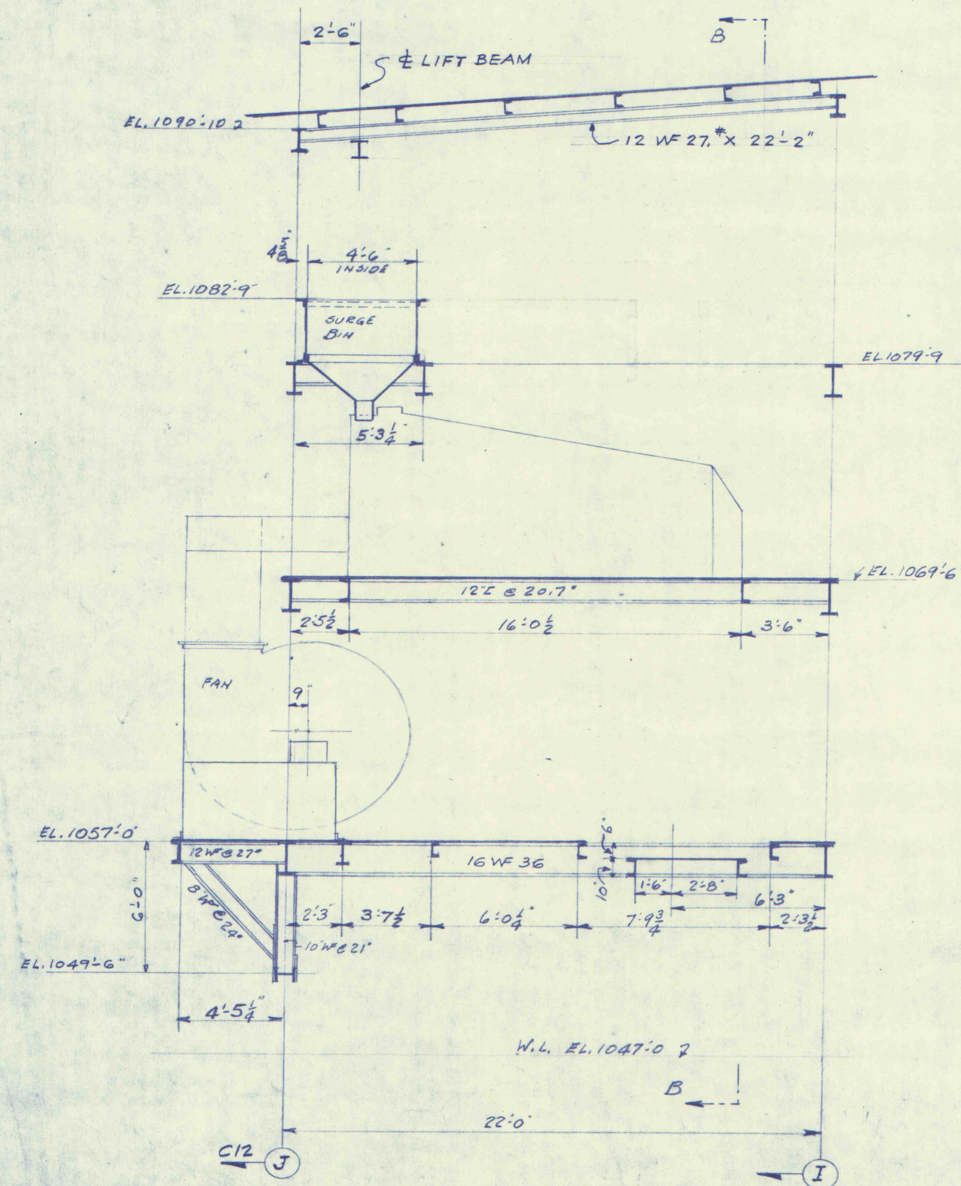
SECTIONAL ELEVATION AT AA DWG. 5636-C9
