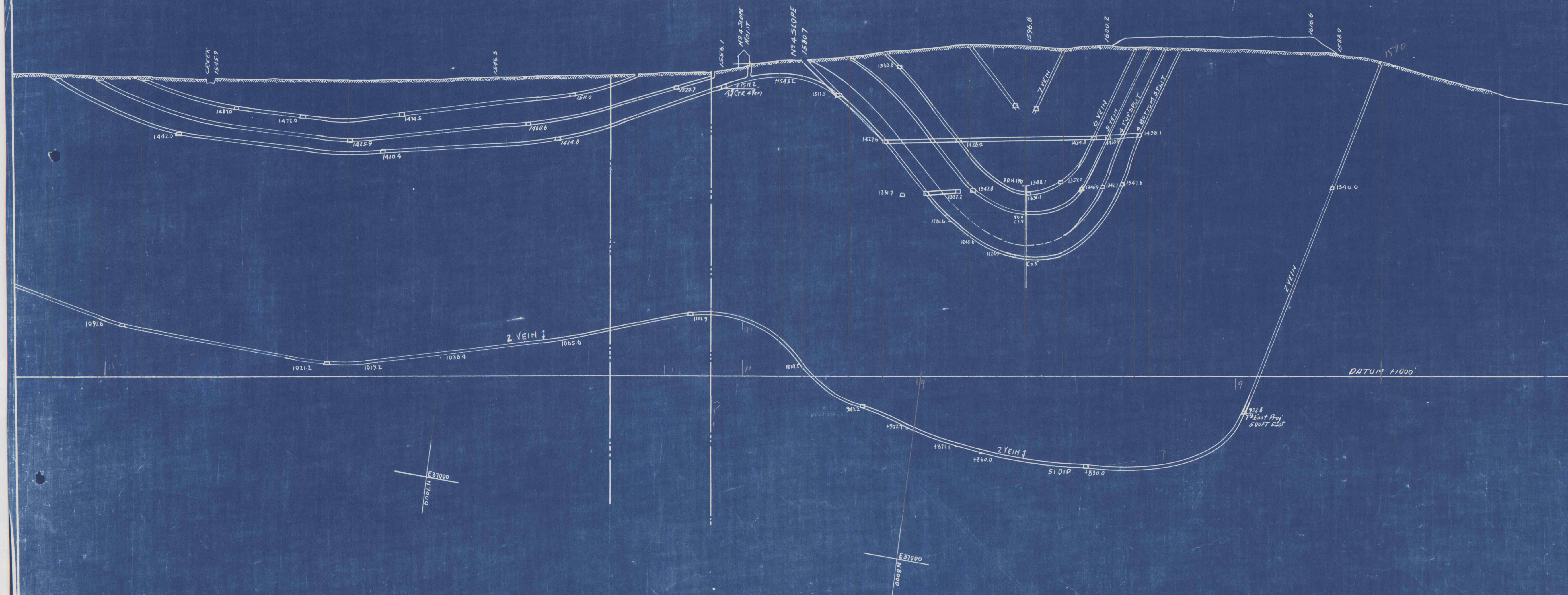
SECTION NO 18A ON LINE OF NO 4 W.A. SLOPE NATALIE COLLIERY COLONIAL COLLIERY COMPANY SCALE-1-IN=100-FT. MAY-1930
