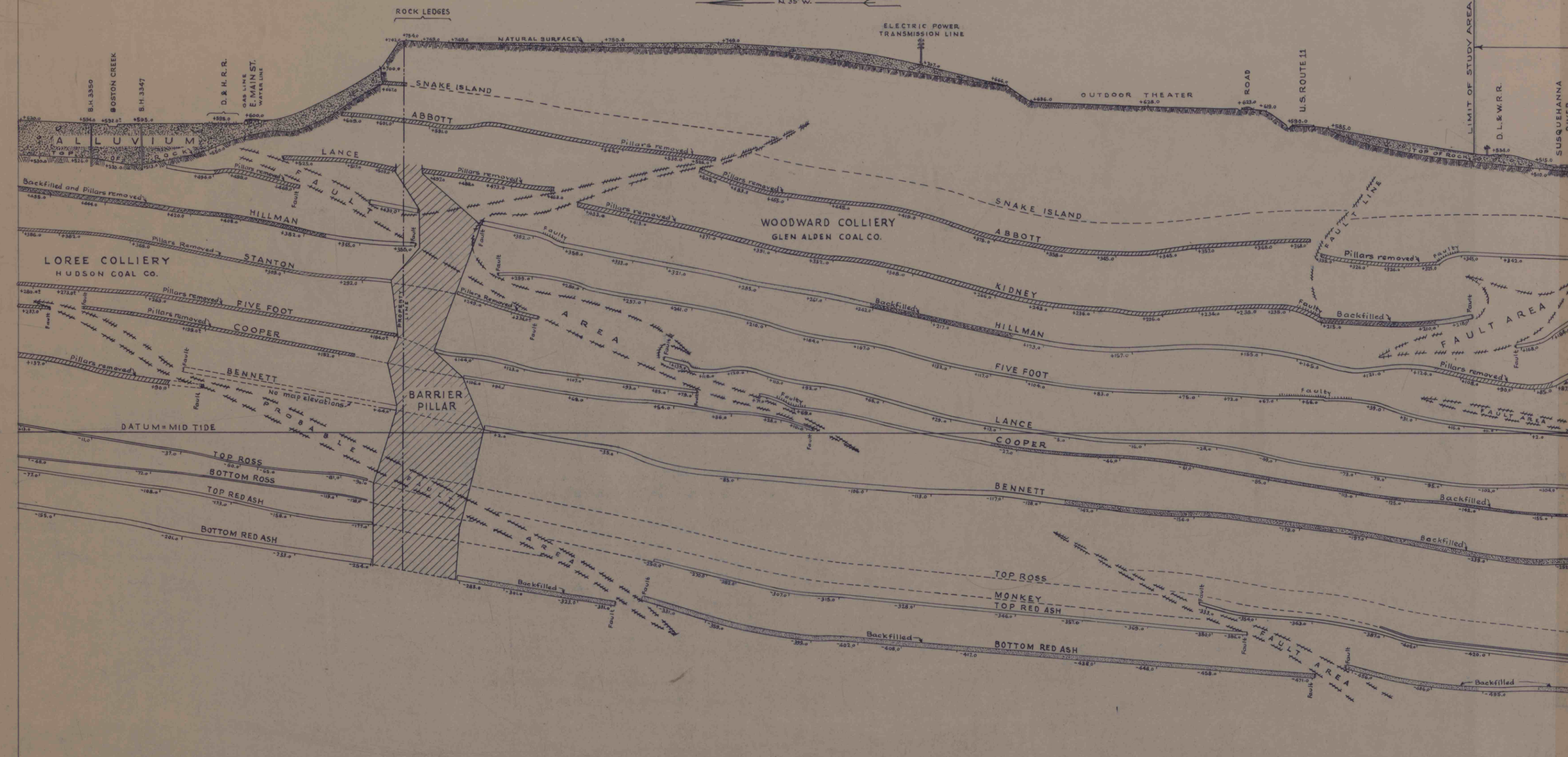
CROSS SECTION FOLIO 30 LOOKING UPSTREAM 0 50 100 200 Horizontal Scale in Feet
