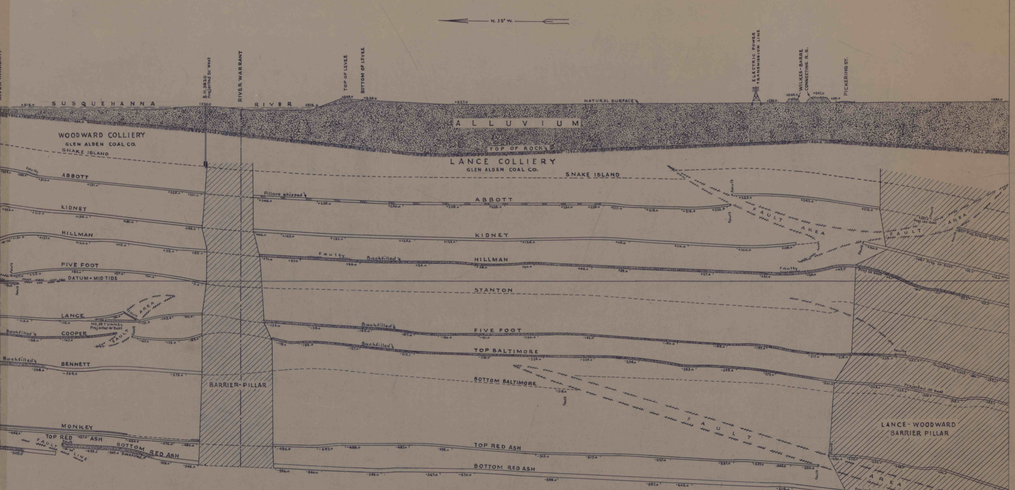
CROSS SECTION FOLIO 3E LOOKING UPSTREAM 0 50 100 200 Horizontal Scale in Feet
