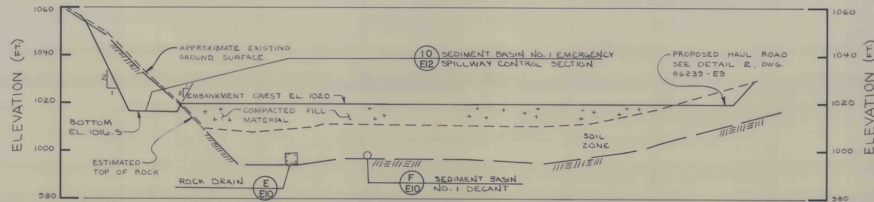
SECTION H-H SEDIMENT BASIN NO. 1 EMBANKMENT CREST SCALE: 1" = 20'
