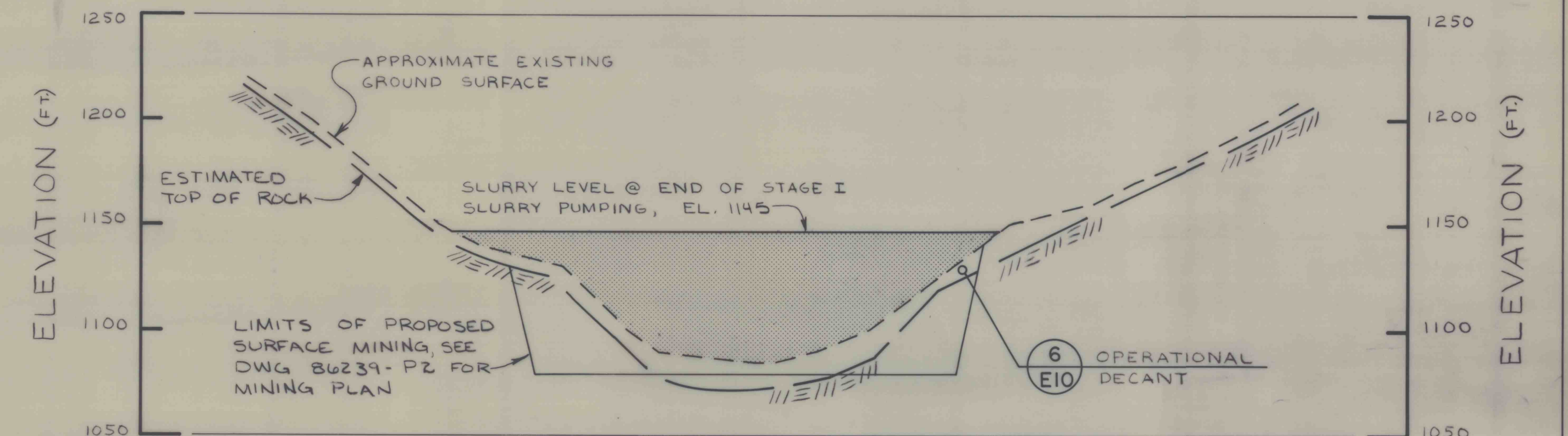
SECTION L-L SECTION THROUGH IMPOUNDMENT SCALE: 1" = 50'
