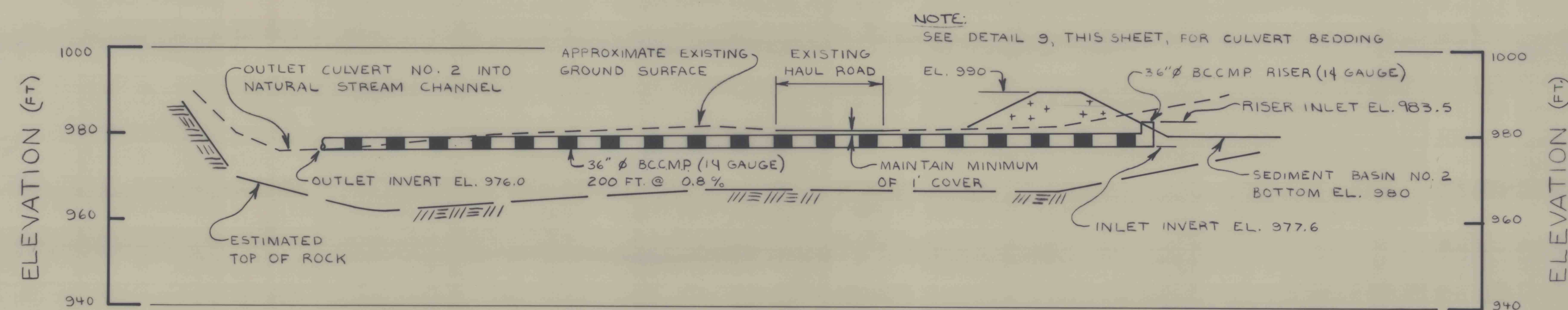
SECTION J-J CULVERT NO. 2 SCALE: 1" = 20'
