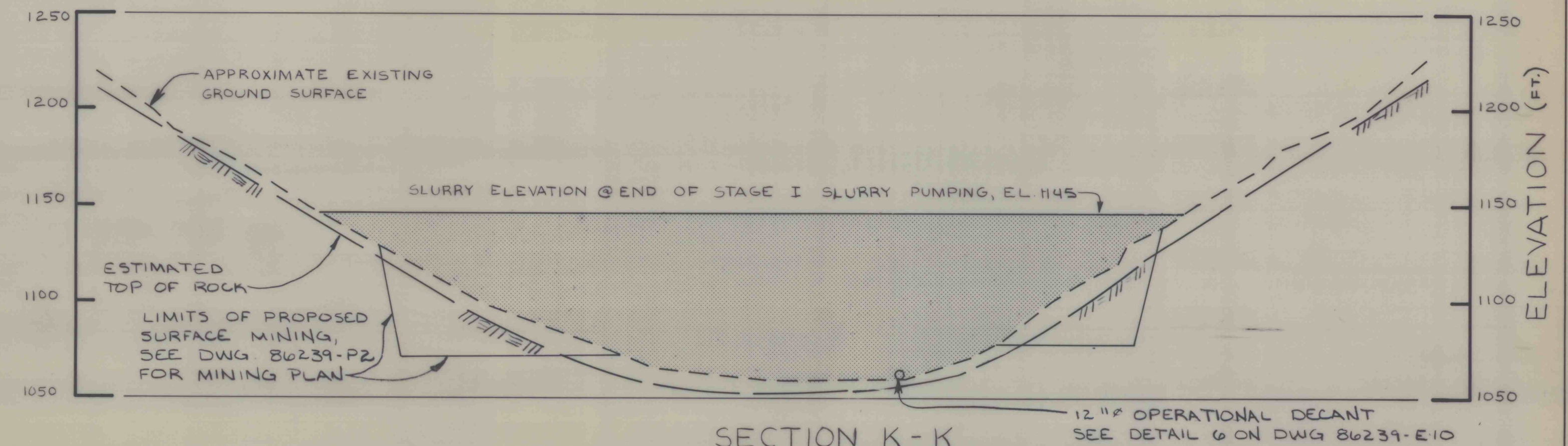
SECTION K-K SECTION THROUGH IMPOUNDMENT SCALE: 1" = 50'
