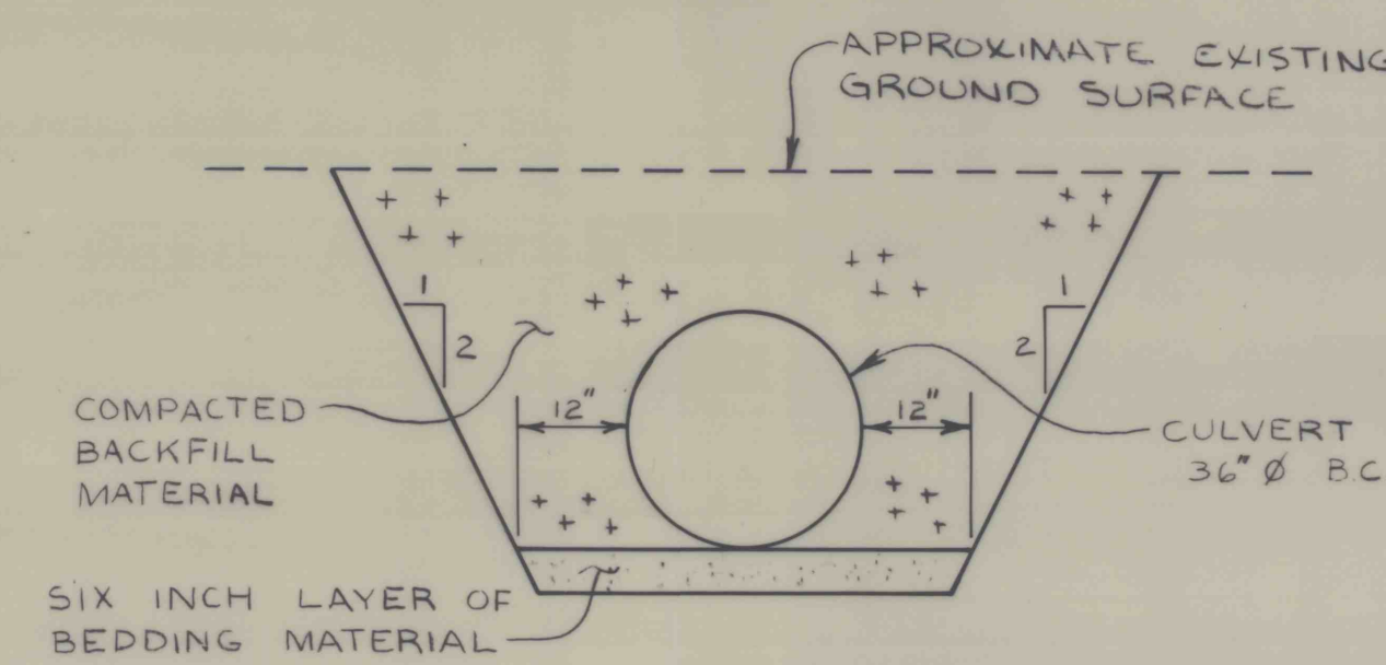
DETAIL 9 TYPICAL CULVERT BEDDING N.T.S.
