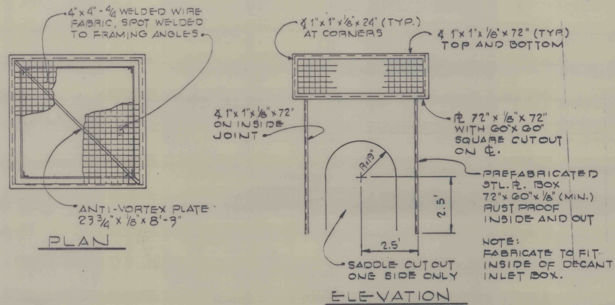
DETAIL 5 REMOVABLE TRASH RACK FOR DECANT INLET BOX N.T.S.
