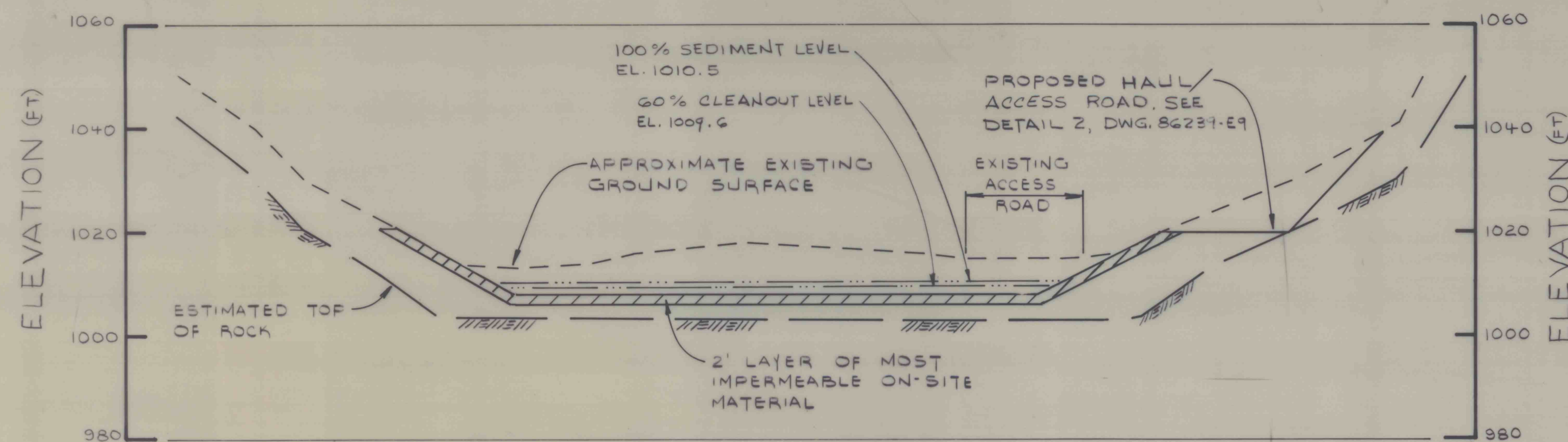
SECTION G-G SEDIMENT BASIN NO. 1 SCALE: 1" = 20'
