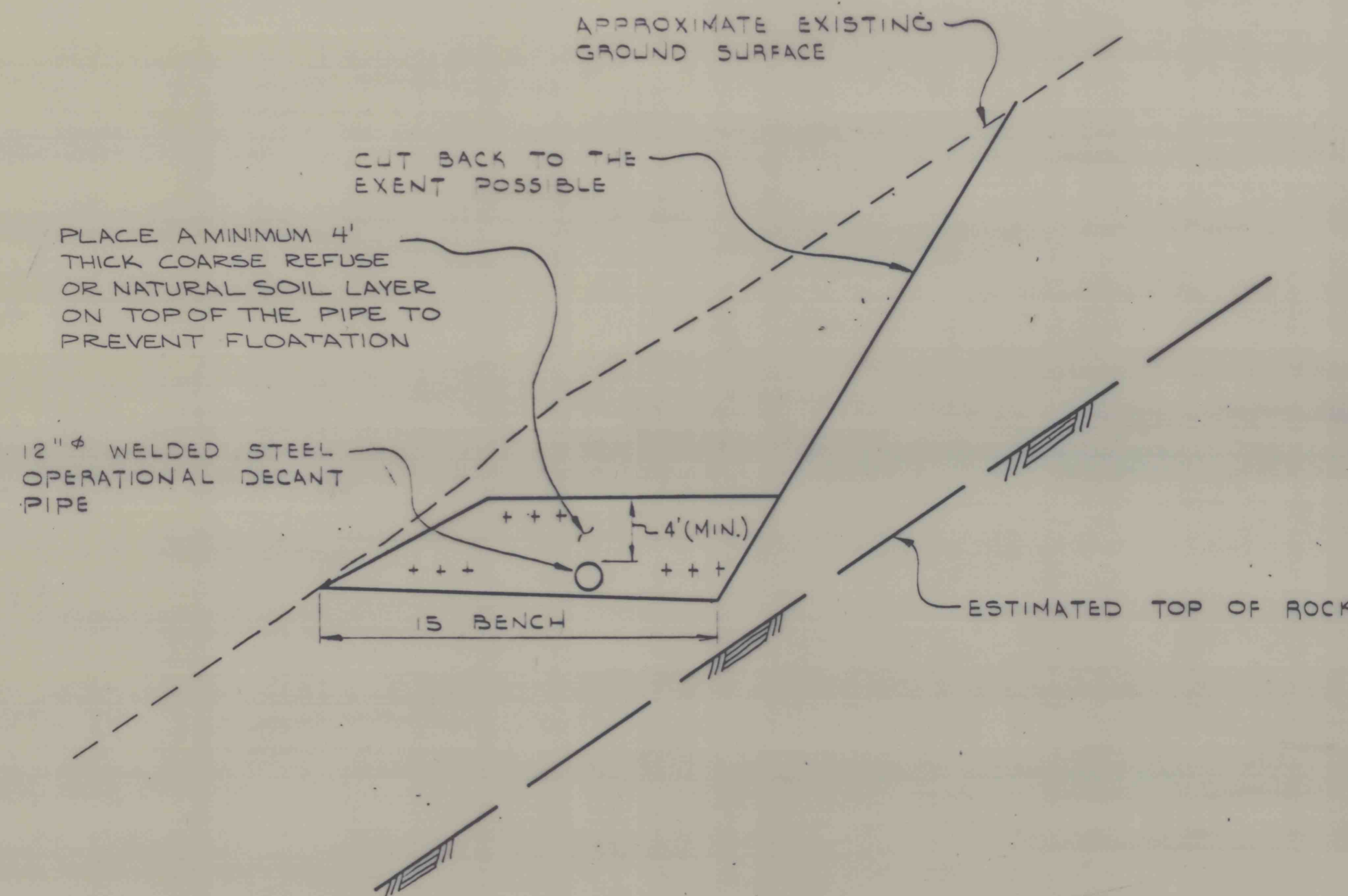
DETAIL 6 OPERATION DECANT INSTALLATION N.T.S.
