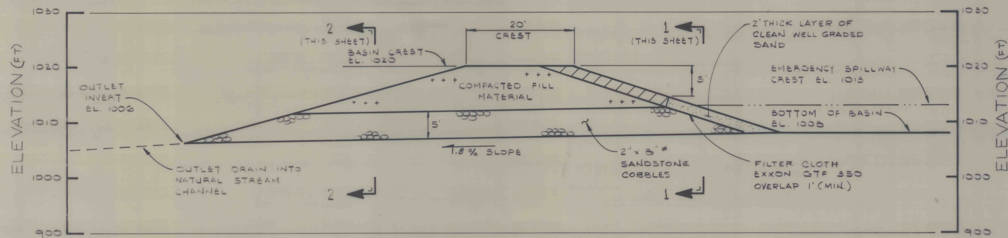
SECTION E-E PROFILE OF ROCK DRAIN AND SEDIMENT BASIN NO. 1 EMBANKMENT SCALE: 1" = 10'
