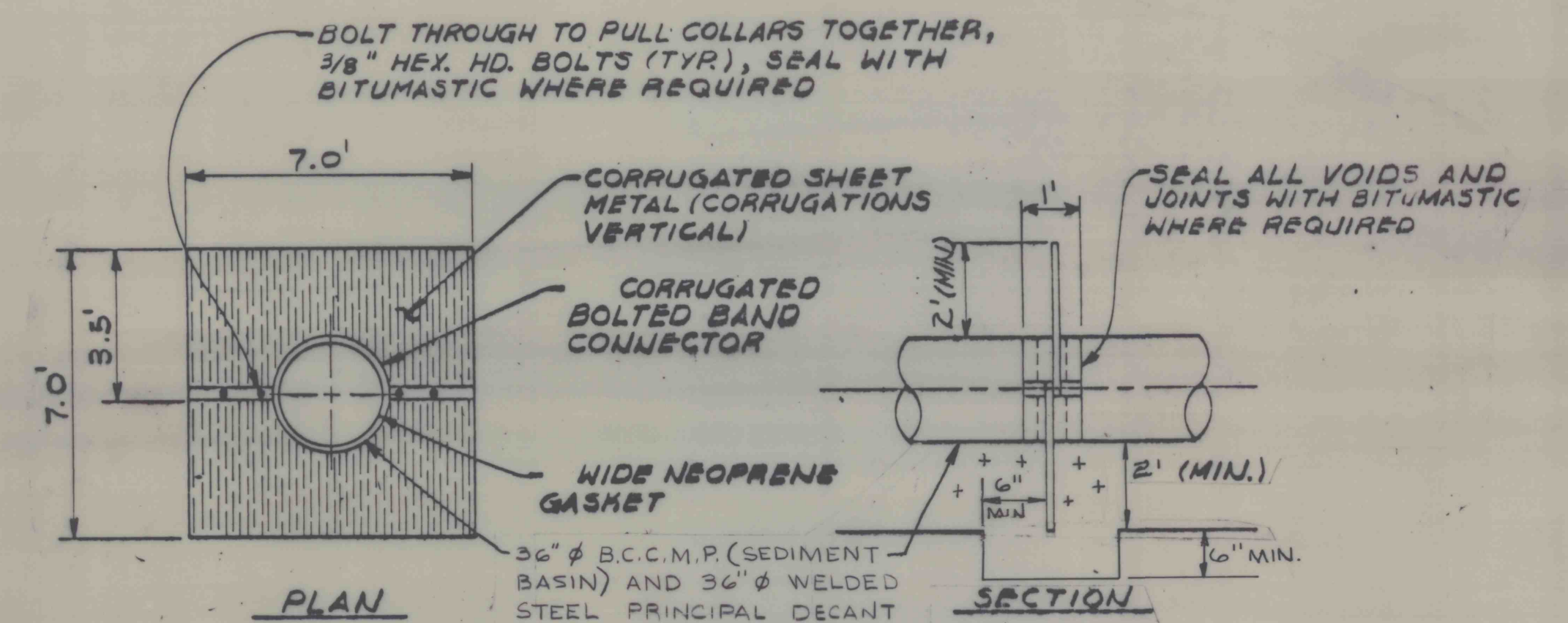
DETAIL 7 DECANT ANTI-SEEP COLLAR N.T.S.
