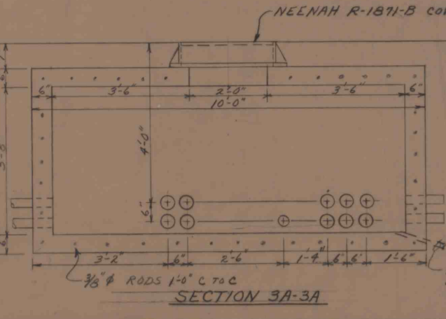
SECTION 3A-3A
