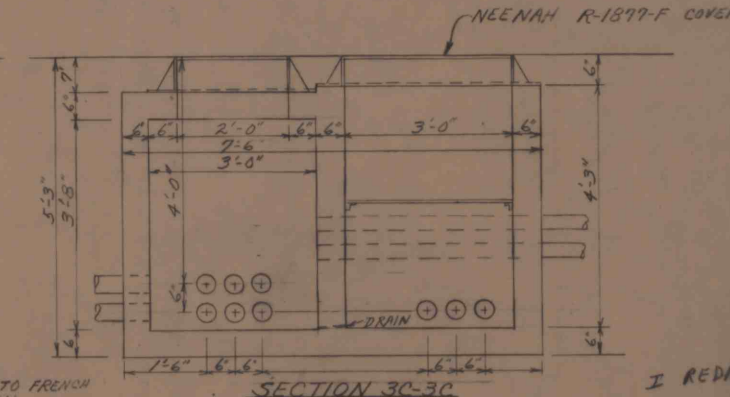
SECTION 3C-3C
