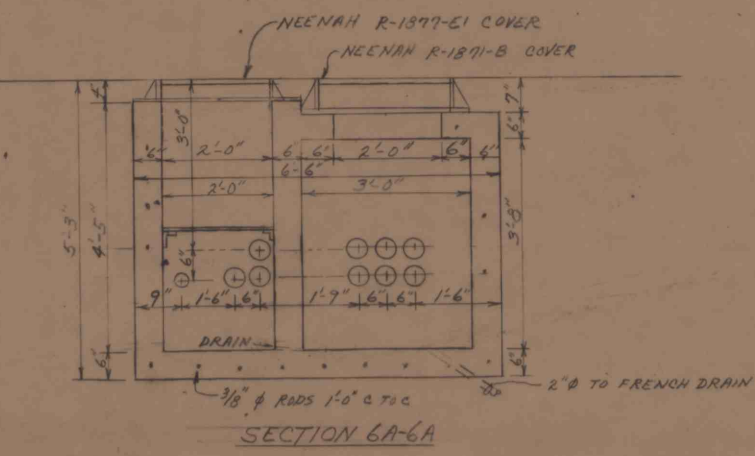
SECTION 6A-6A
