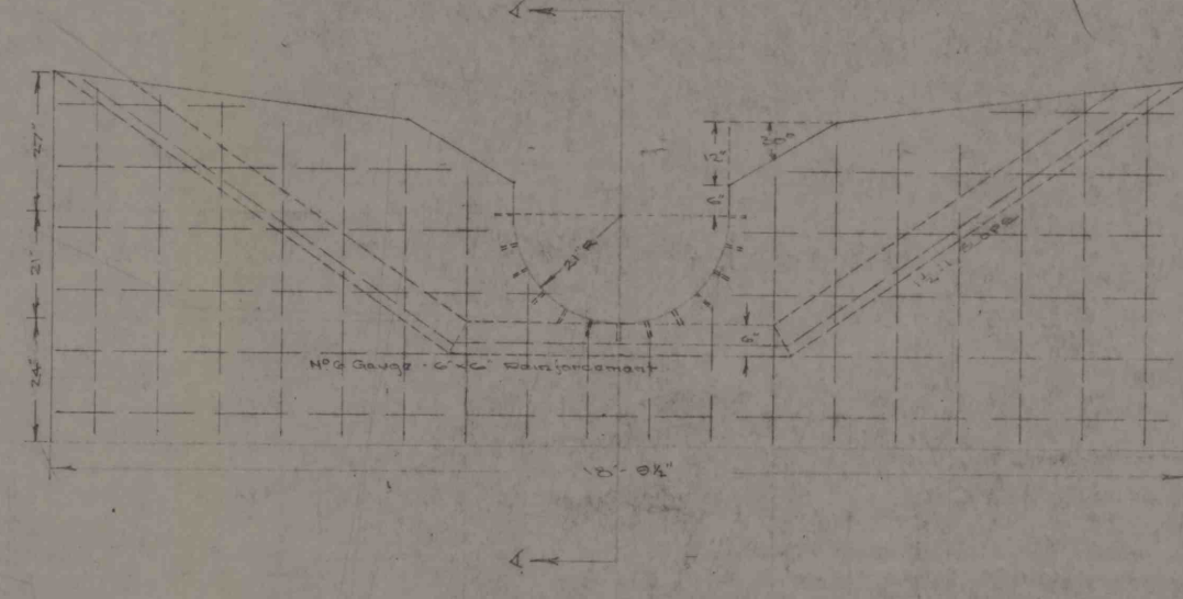
FIGURE 2 END WALL AND APRON DETAIL FOR 12\"/>
