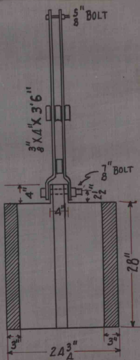
FRONT ELEVATION
